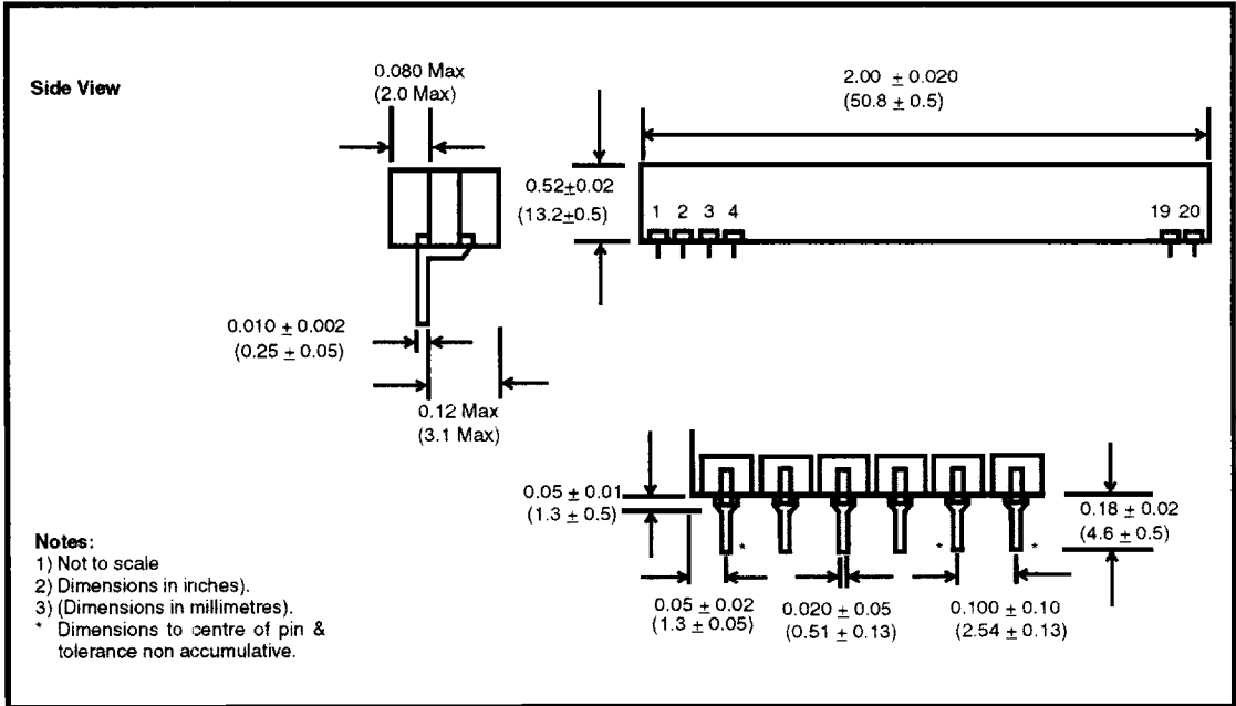
Figure 4 - Mechanical Data
