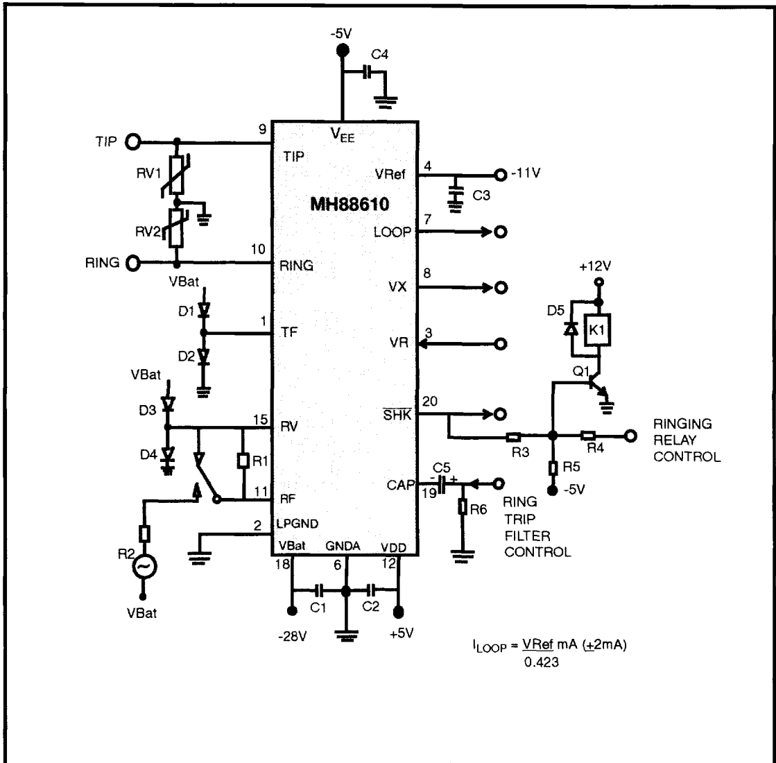
Figure 3 - Application Circuit
