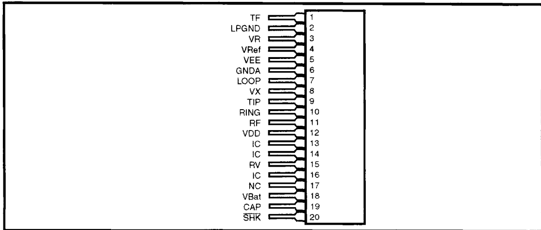
Figure 2 - Pin Connections
