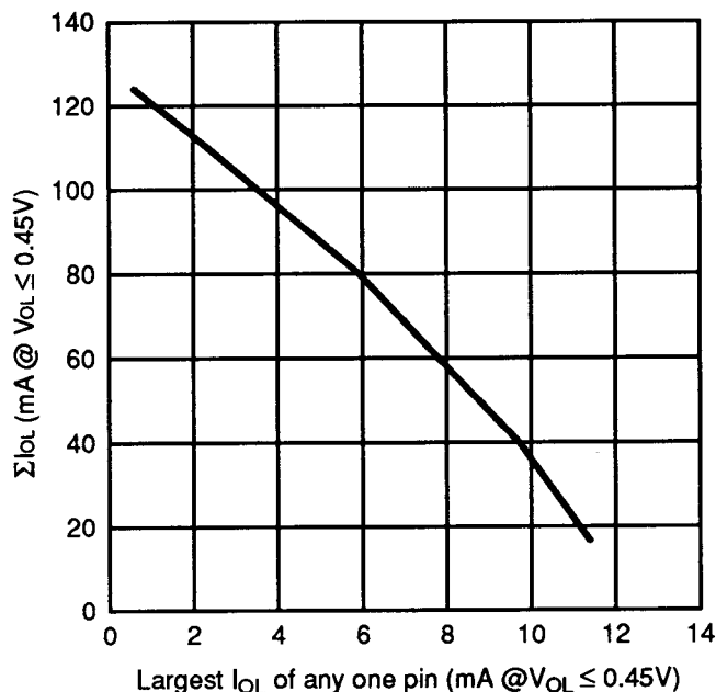
Fig. 3 – \Sigma I_{OL} vs I_{OL} (@ V_{OL} \leq 0.45V )
