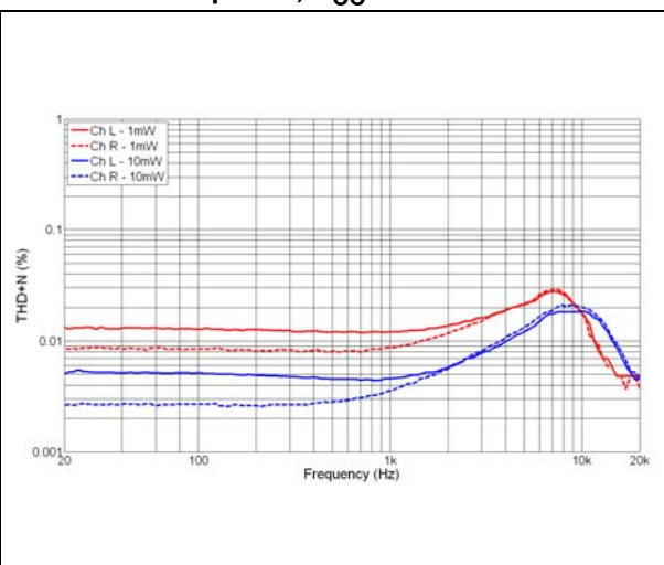
Figure 45. THD+N vs. frequency, R_L = 32\ \Omega , in-phase, V_{CC} = 4.8\text{ V}
