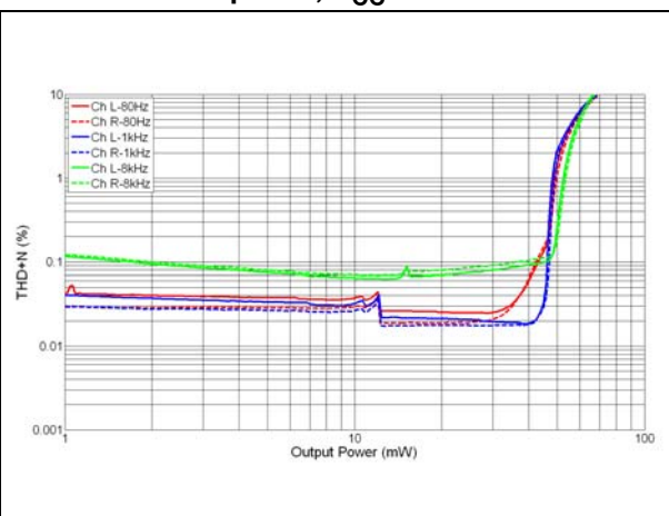
Figure 15. THD+N vs. output power - R_L = 16 \Omega , in-phase, V_{CC} = 4.8 \text{ V}
