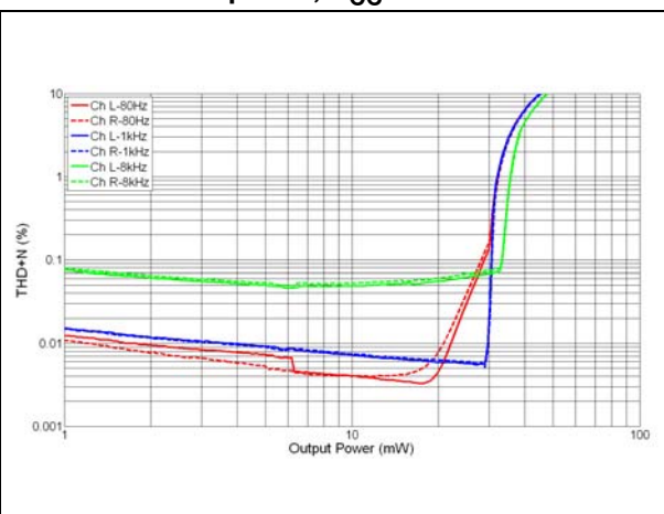
Figure 17. THD+N vs. output power - R_L = 32 \Omega , in-phase, V_{CC} = 2.5 \text{ V}
