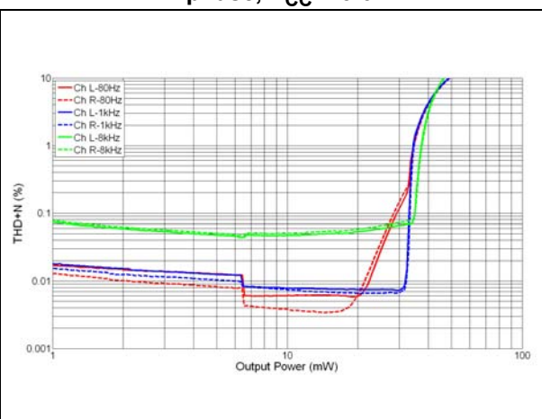
Figure 19. THD+N vs. output power - R_L = 32 \Omega , in-phase, V_{CC} = 3.6 \text{ V}
