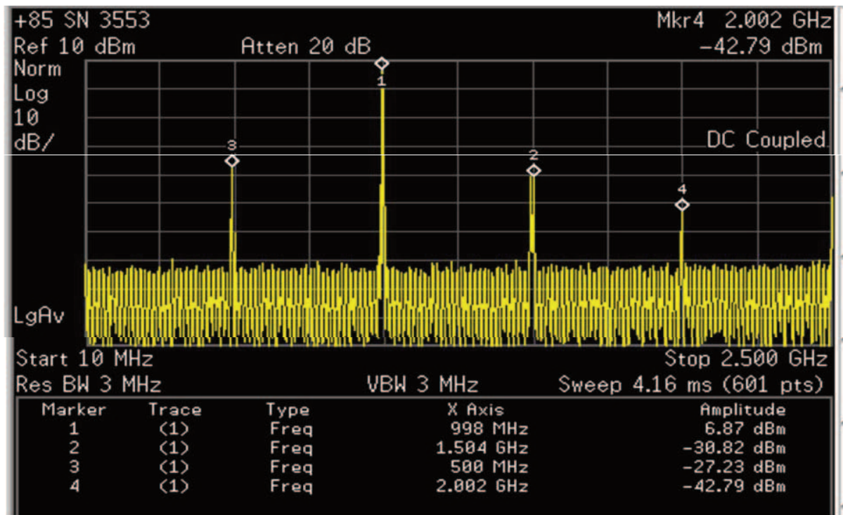
Output power spectrum including sub-harmonics of a 1GHz SO at +85°C
