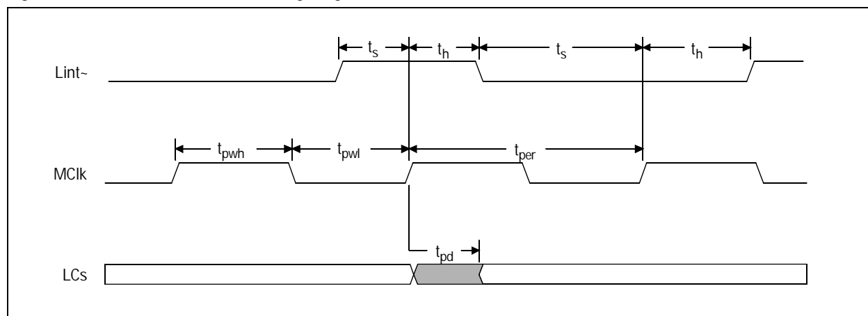
Figure 4-7. Framers (Line) Control Timing Diagram
