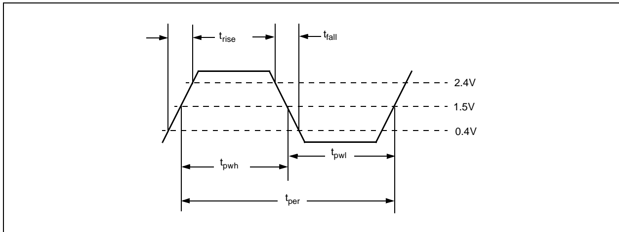
Figure 4-2. Output Waveform
