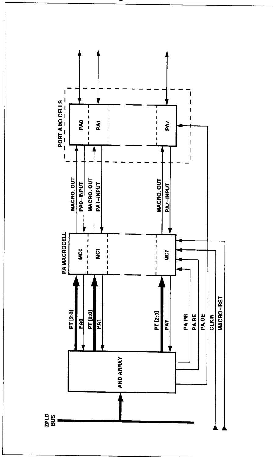
Figure 13. PA Macrocell Block Diagram
