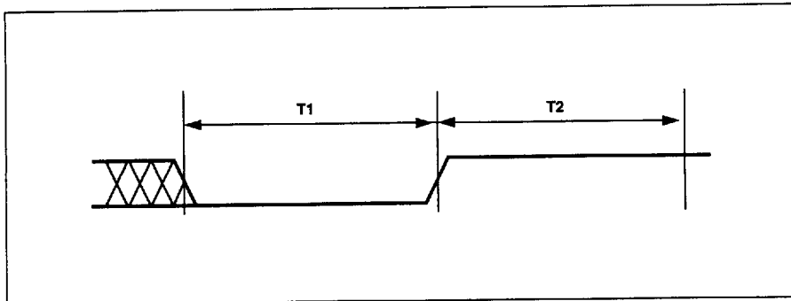
Figure 47. Reset Timing
