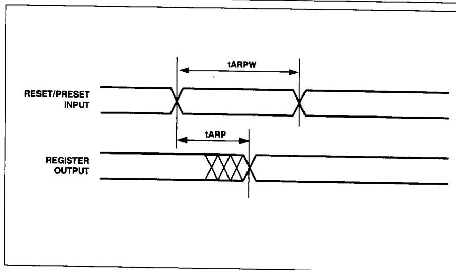
Figure 46. Asynchronous Reset/Preset
