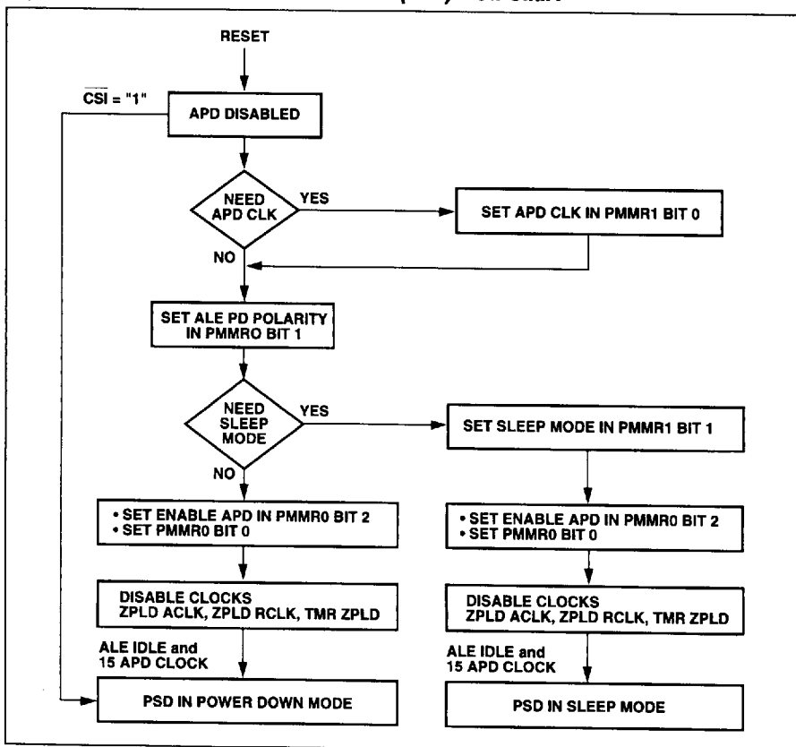
Figure 36a. Automatic Power Down Unit (APD) Flow Chart
