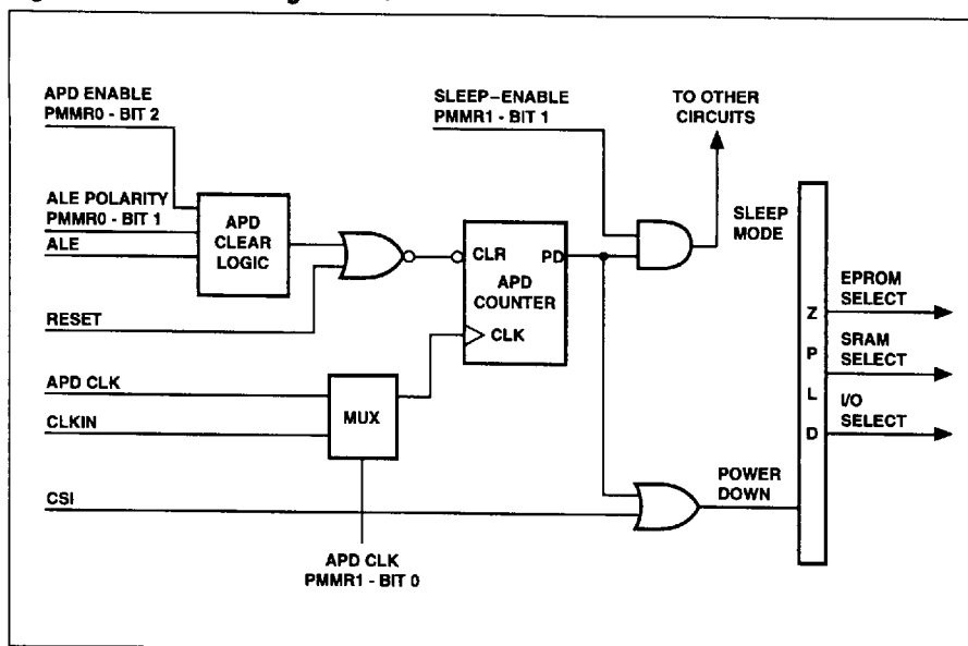
Figure 36. Power Management Unit
