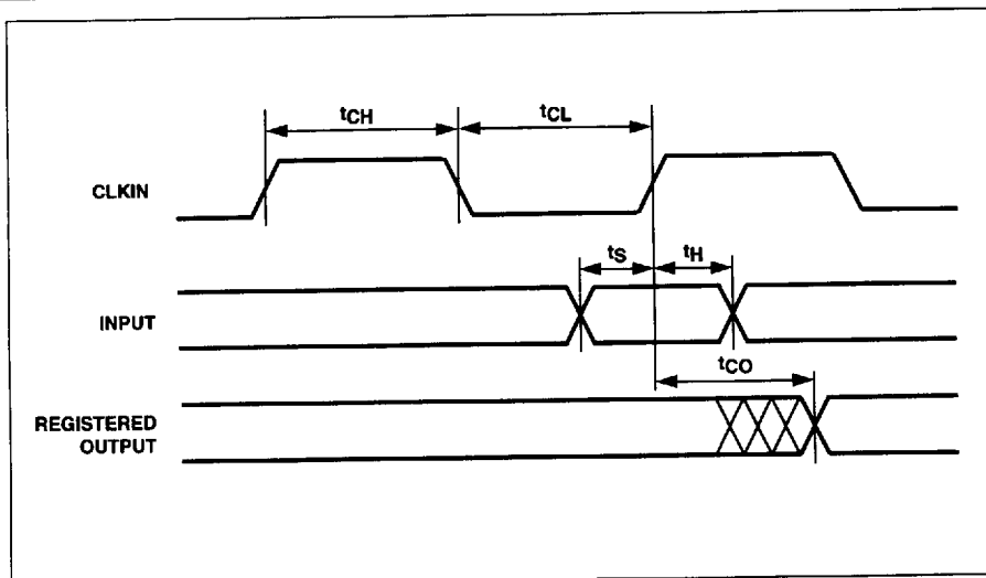
Figure 43. Synchronous Clock Mode Timing – ZPLD
