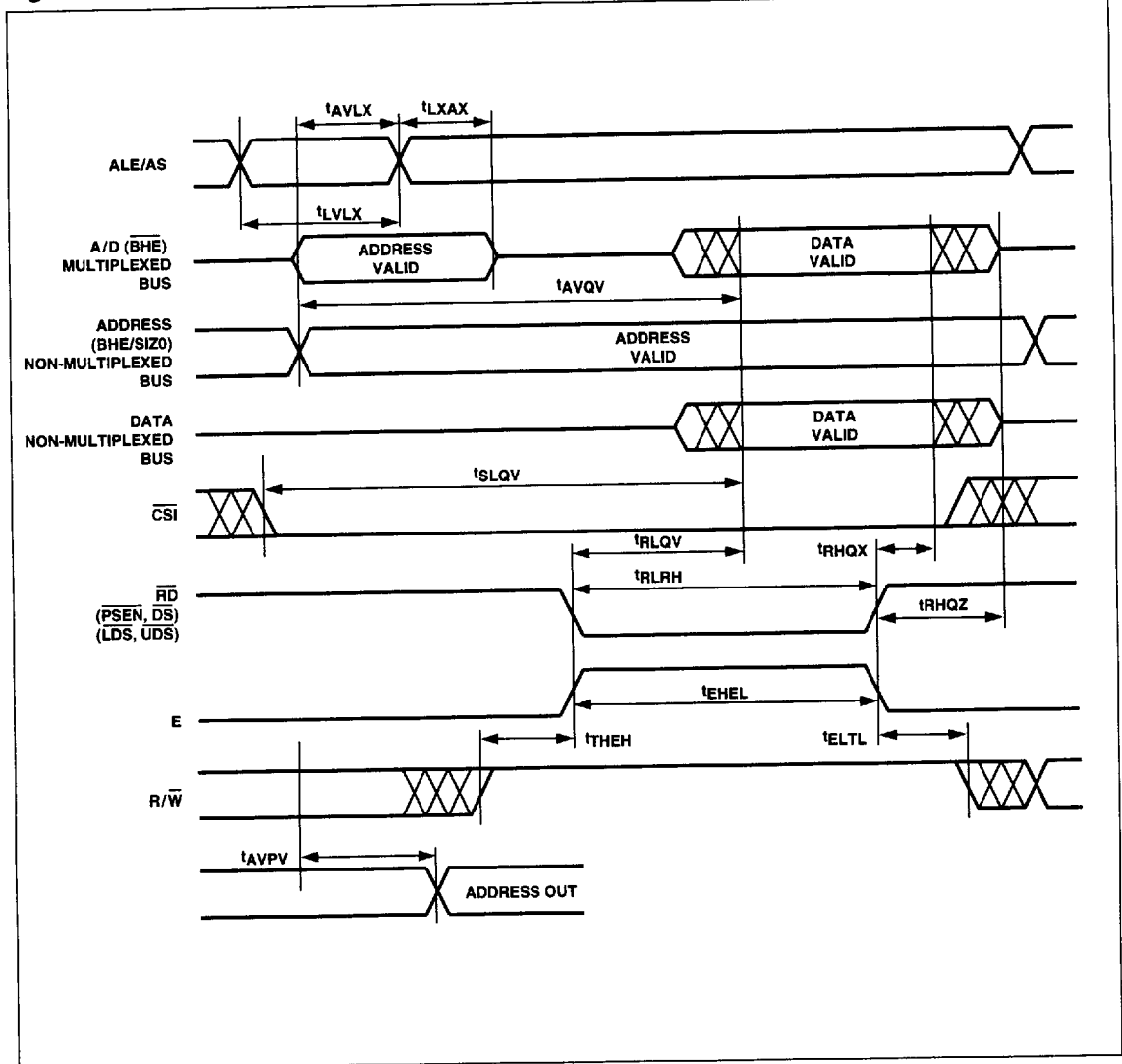
Figure 38. Read Timing
