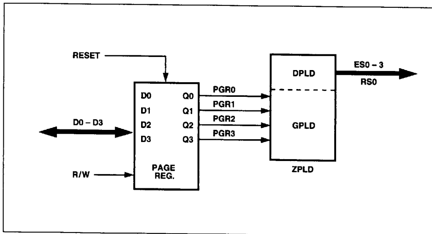
Figure 35. Page Register
