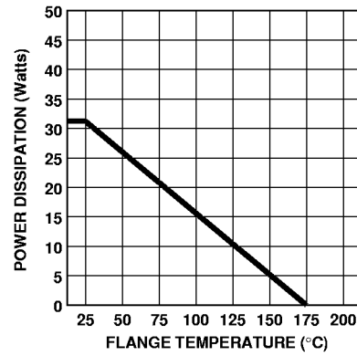
Figure 2. IM5053-4L Maximum Total Power Dissipation vs. Flange Temperature.
