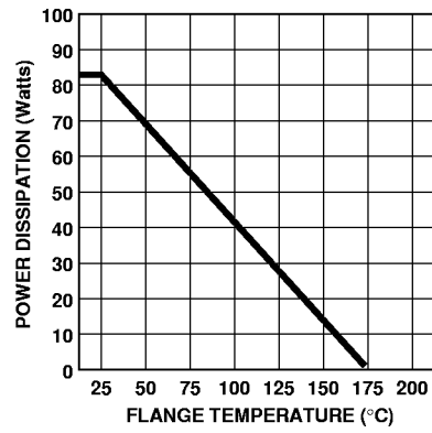
Figure 6. IM5053-16L Maximum Total Power Dissipation vs. Flange Temperature.
