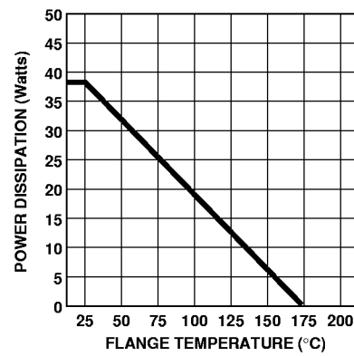
Figure 4. IM5053-8L Maximum Total Power Dissipation vs. Flange Temperature.
