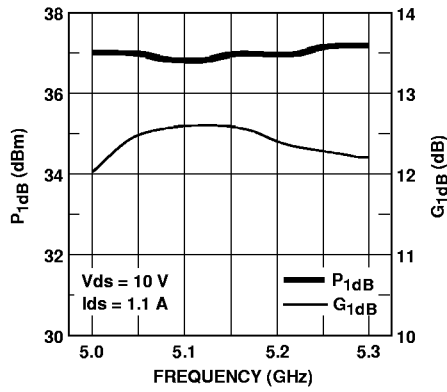
Figure 1. IM5053-4L Output Power, Gain vs. Frequency.
