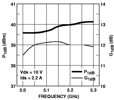
Figure 3. IM5053-8L Output Power, Gain vs. Frequency.
