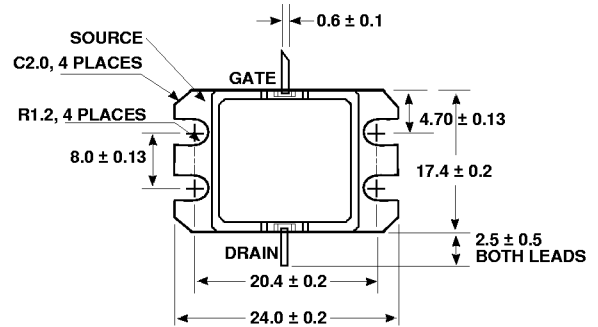
C24A Package Outline IM5053-16L and IM5053-32L
