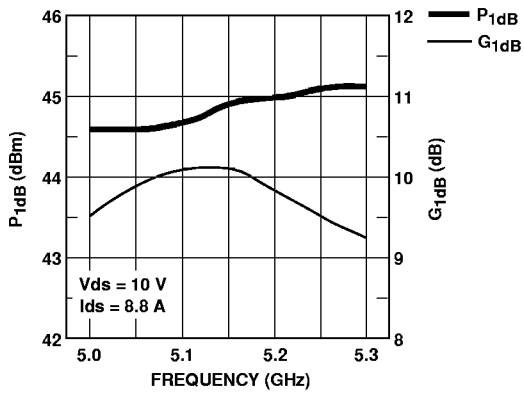
Figure 7. IM5053-32L Output Power, Gain vs. Frequency.
