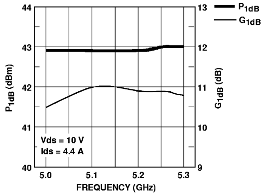
Figure 5. IM5053-16L Output Power, Gain vs. Frequency.
