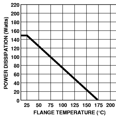
Figure 8. IM5053-32L Maximum Total Power Dissipation vs. Flange Temperature.
