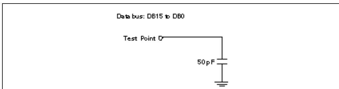
Figure 59 Load Circuit
