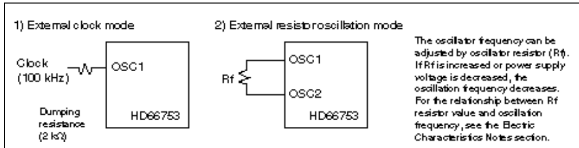
Figure 32 Oscillation Circuits
