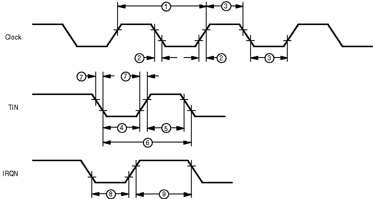
Additional Timing
