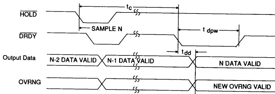
Conversion Timing
