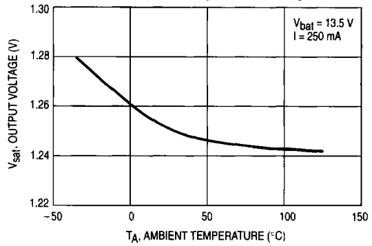
Figure 6. Output Voltage versus Temperature
