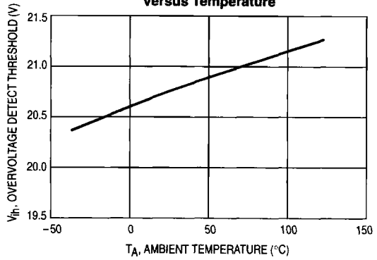
Figure 4. Overvoltage Detection versus Temperature
