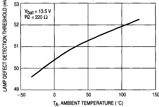
Figure 7. Defect Lamp Detection versus Temperature
