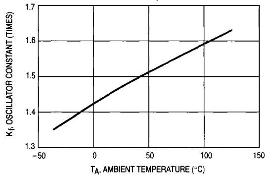
Figure 8. Oscillator Constant versus Temperature
