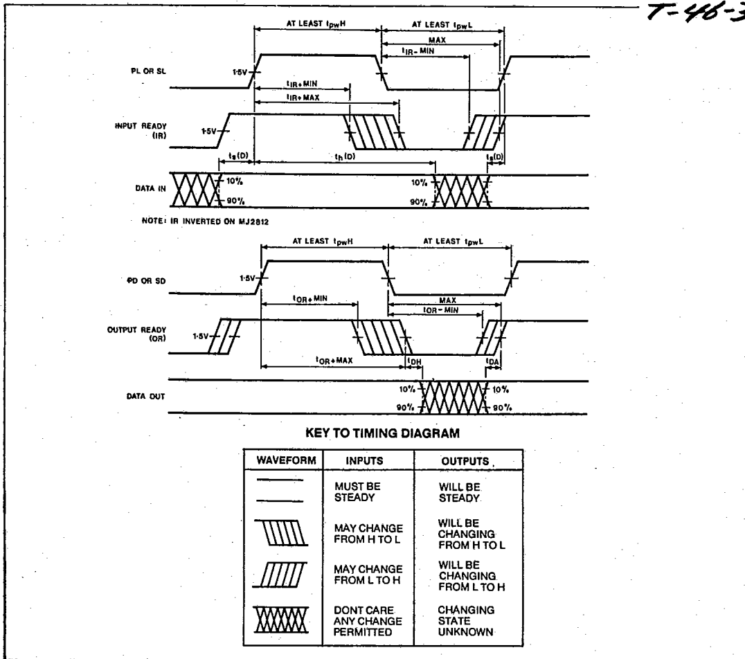
Fig. 6 Timing diagram
