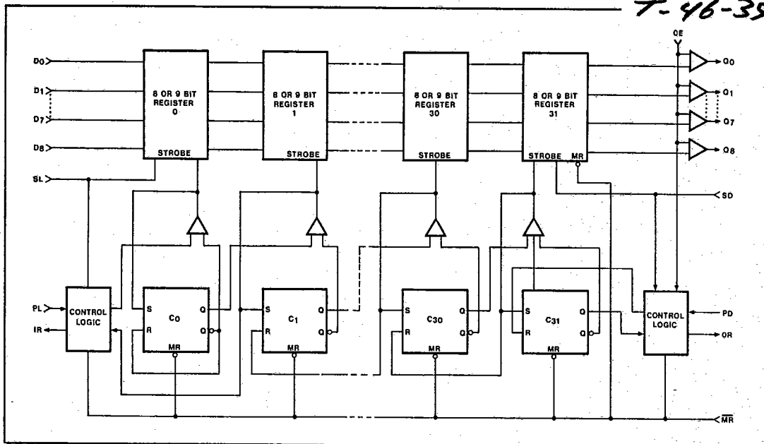
Fig. 4 Logic block diagram
