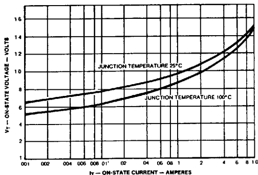
9. ON-STATE CHARACTERISTICS
