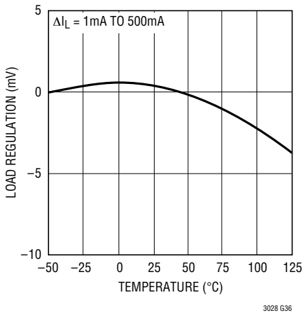
Output 1 Load Regulation
