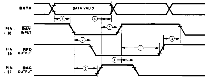
Figure 50. 3-Wire Handshake Input
