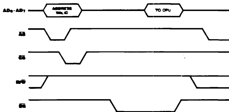
Figure 6. Z-BUS Read Cycle Timing
