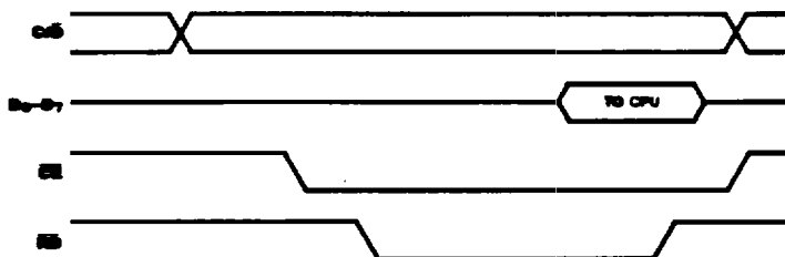
Figure 9. Non-Z-BUS Read Cycle Timing
