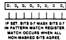
Figure 31. Pattern Mask Register
