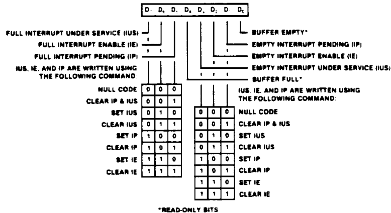
Figure 27. Interrupt Status Registers (Continued)
