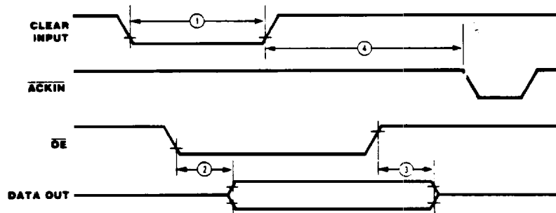
Figure 47. Port 2 Side Operation
