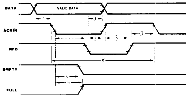
Figure 49. 2-Wire Handshake (Port 2 Side Only) Input
