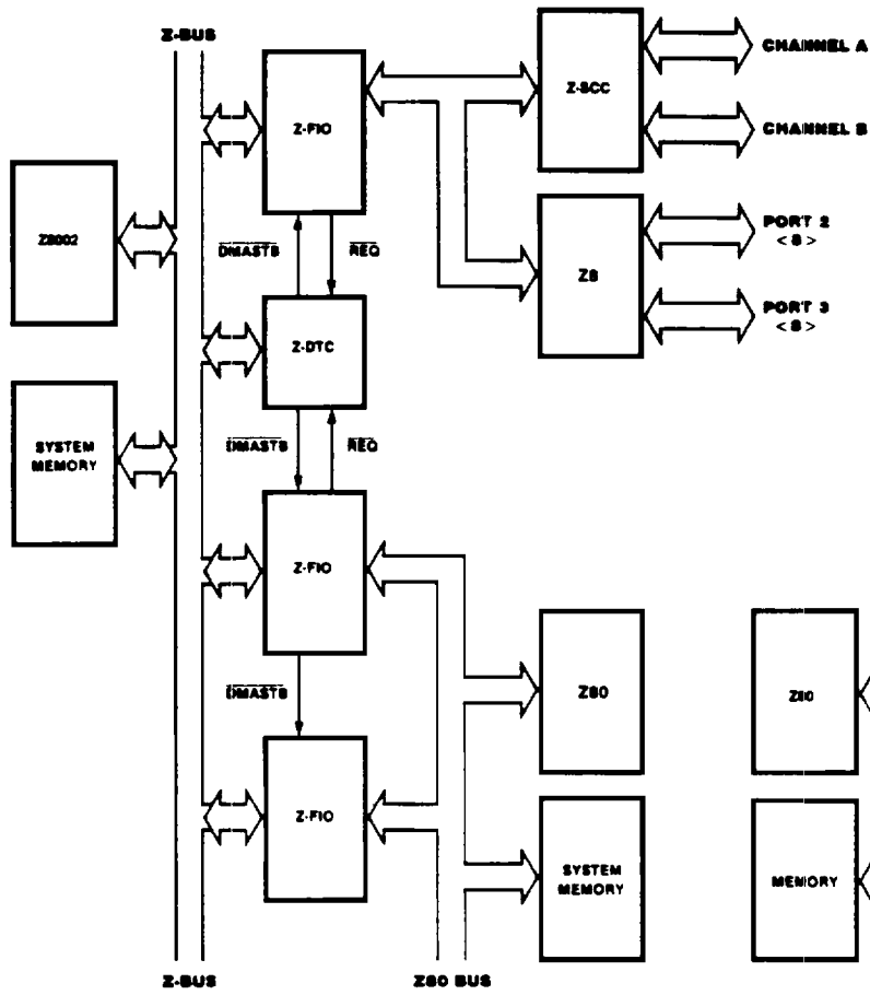
Figure 4. CPU to CPU Configuration
