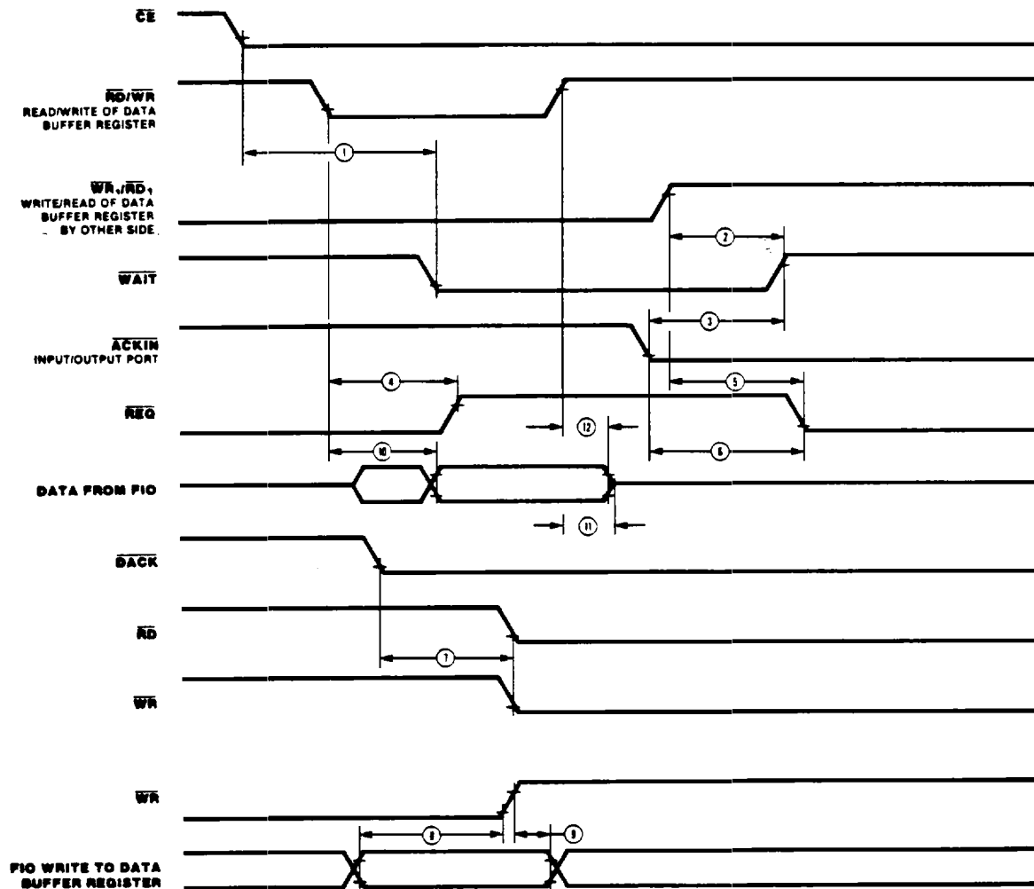
Figure 45. Non-Z-BUS Request/Wait Timing
