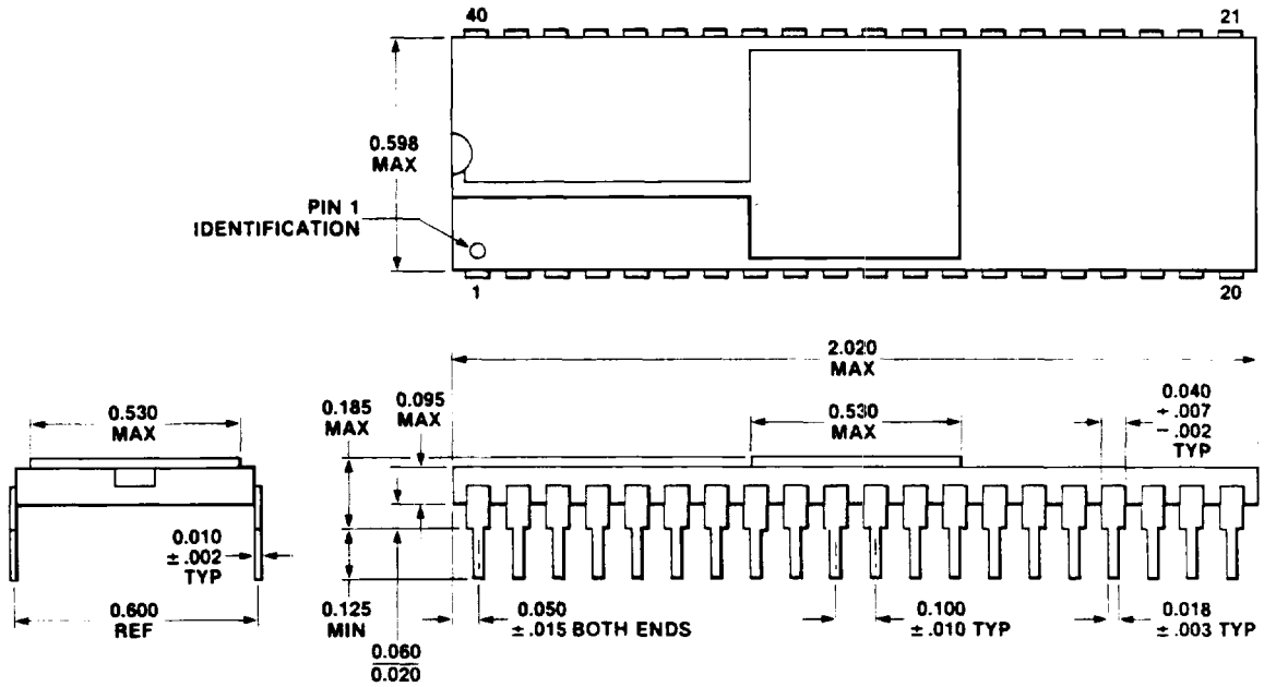
40-Pin Ceramic Dual In-line Package (DIP)
