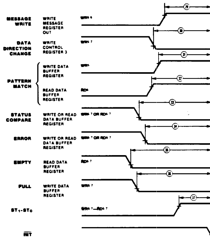
Figure 44. FIO Non-Z-BUS Interrupt Timing
