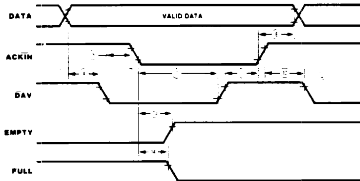
Figure 48. 2-Wire Handshake (Port 2 Side Only) Output
