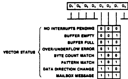
Figure 29. Interrupt Vector Register
