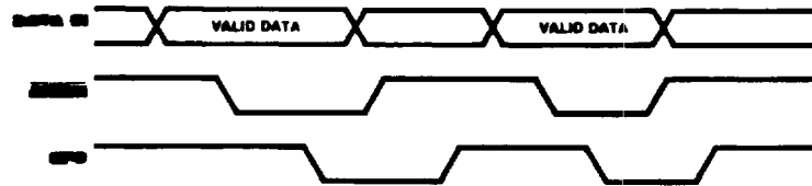
Figure 21. Interlocked Handshake Timing (Input) Port 2 Side Only
