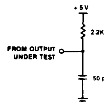
Open-Drain Test Load
