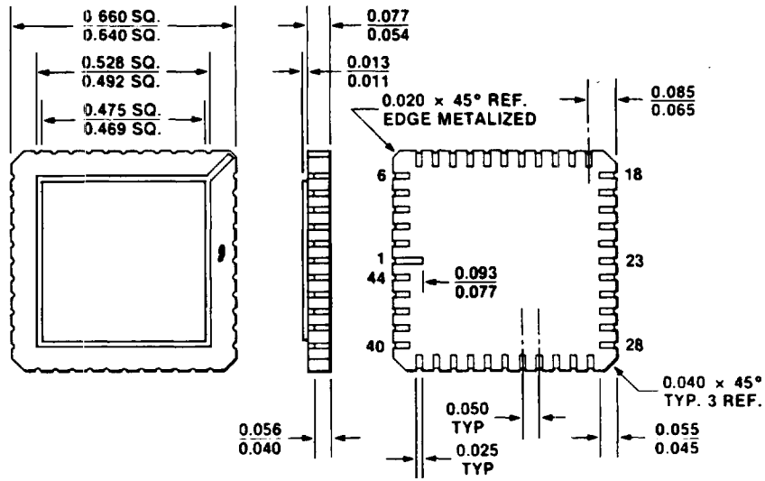
44-Pin Ceramic Leadless Chip Carrier (LCC)
