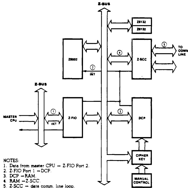
Figure 25. Typical Application: Node Controller
