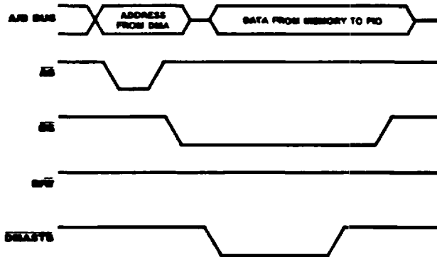
Figure 14. Z-BUS Memory to FIO Data Transaction
