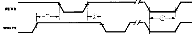
Figure 46. Non-Z-BUS Reset Timing
