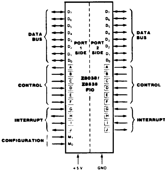
Figure 1. Pin Functions
