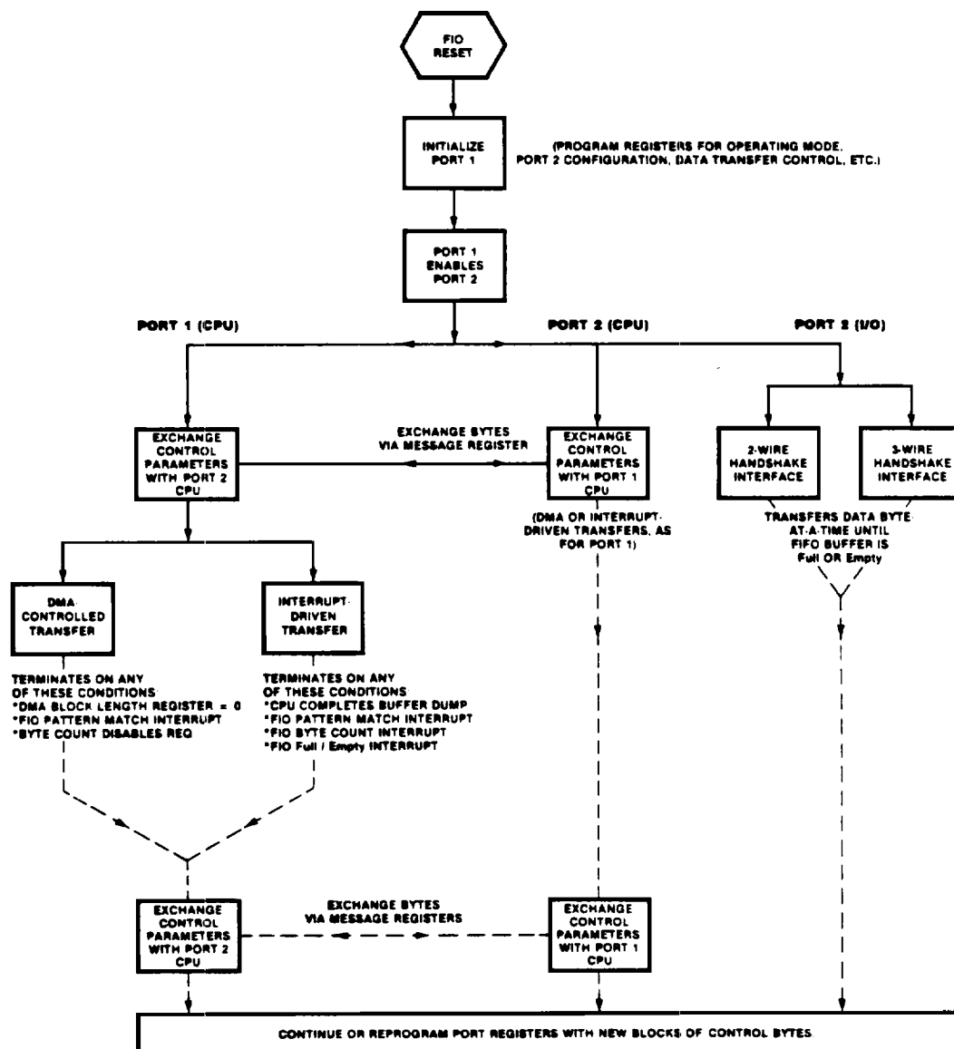
Figure 20. FIO Data Transfer Options
