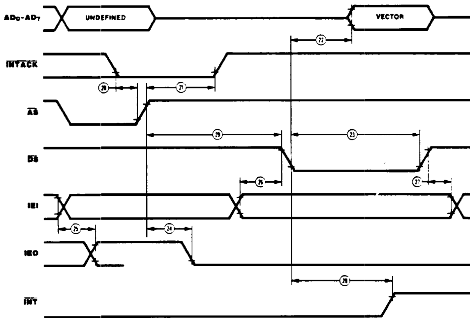
Figure 37. Z-BUS CPU Interrupt Acknowledge Timing
