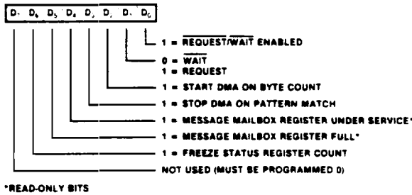
Figure 26. Control Registers
