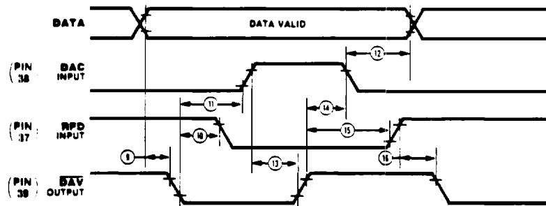
Figure 51. 3-Wire Handshake Output
