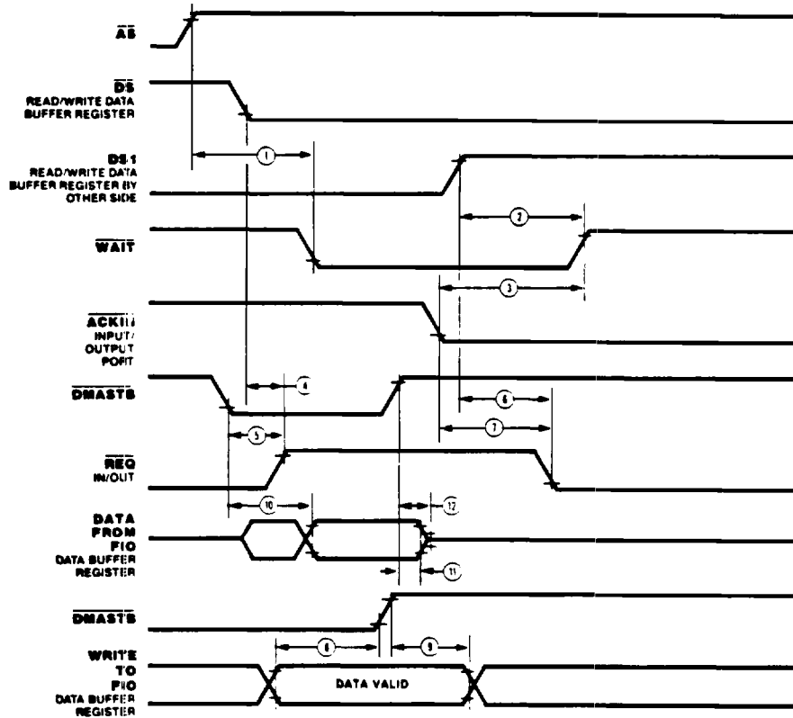
Figure 39. Z-BUS Request/Wait Timing
