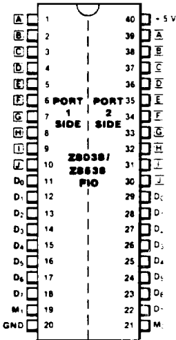
Figure 2a. 40-pin Dual-In-Line Package (DIP) Pin Assignments
