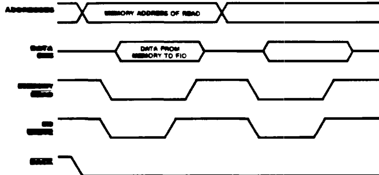
Figure 16. Non-Z-BUS Memory to FIO Data Transaction
