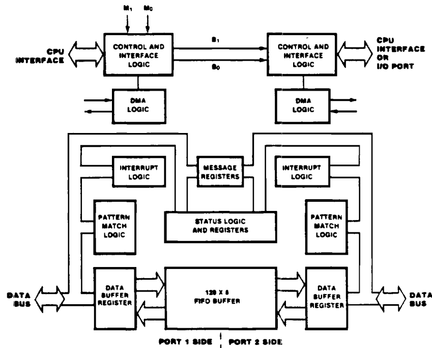
Figure 3. FIO Block Diagram
