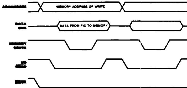
Figure 15. Non-Z-BUS FIO to Memory Transaction
