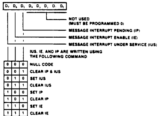
Figure 27. Interrupt Status Registers
