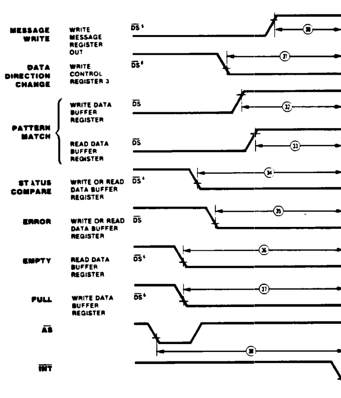
Figure 38. Z-BUS Interrupt Timing
