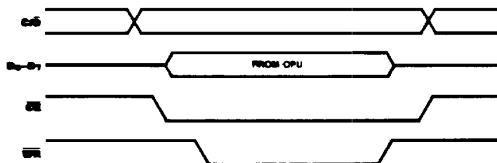
Figure 10. Non-Z-BUS Write Cycle Timing
