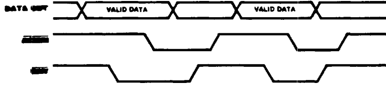
Figure 22. Interlocked Handshake Timing (Output) Port 2 Side Only
