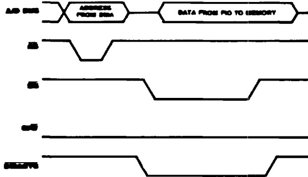
Figure 13. Z-BUS FIO to Memory Data Transaction
