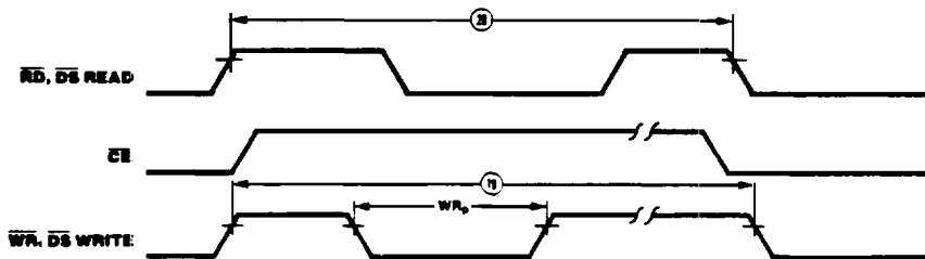
Figure 42. Z-BUS/Non-Z-BUS Recovery Time
