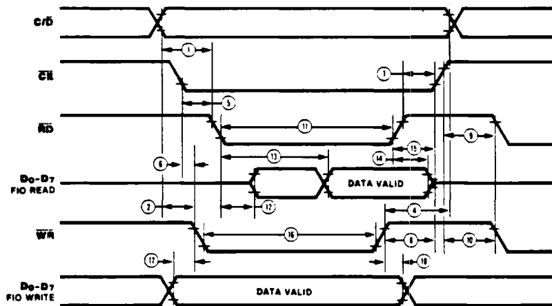
Figure 41. Non-Z-BUS CPU Interface Timing
