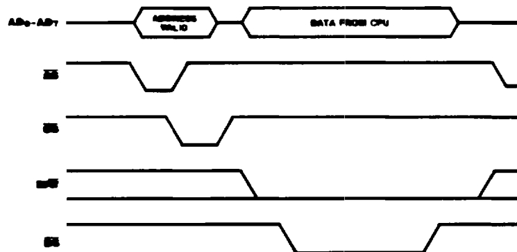
Figure 7. Z-BUS Write Cycle Timing
