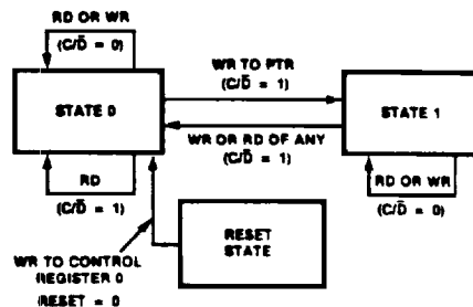
Figure 8. Register Access in Non-Z-BUS Mode
