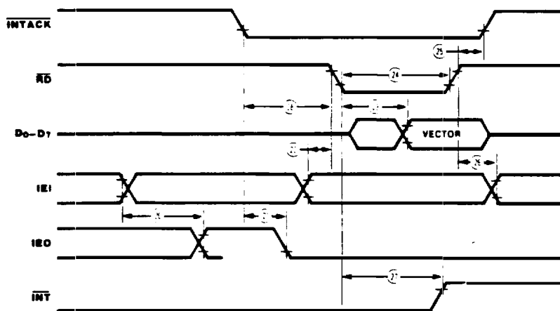
Figure 43. Non-Z-BUS Interrupt Acknowledge Timing
