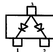
Common Anode
