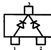
Common Cathode
