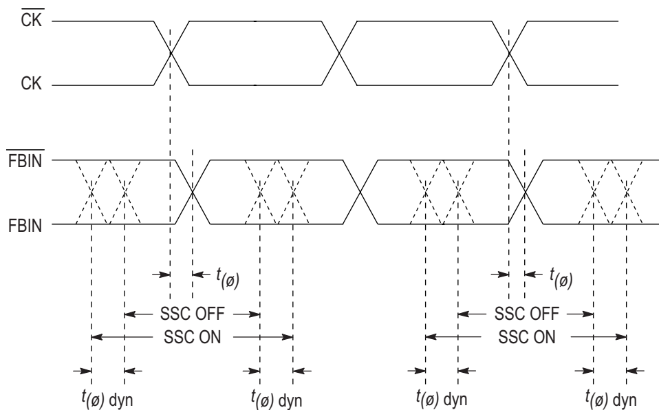
Figure 11. Dynamic Phase Offset
