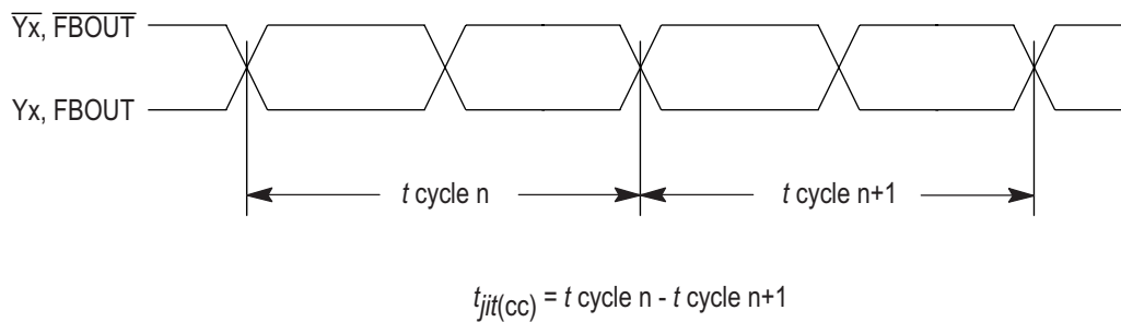
Figure 5. Cycle-to-Cycle Period Jitter
