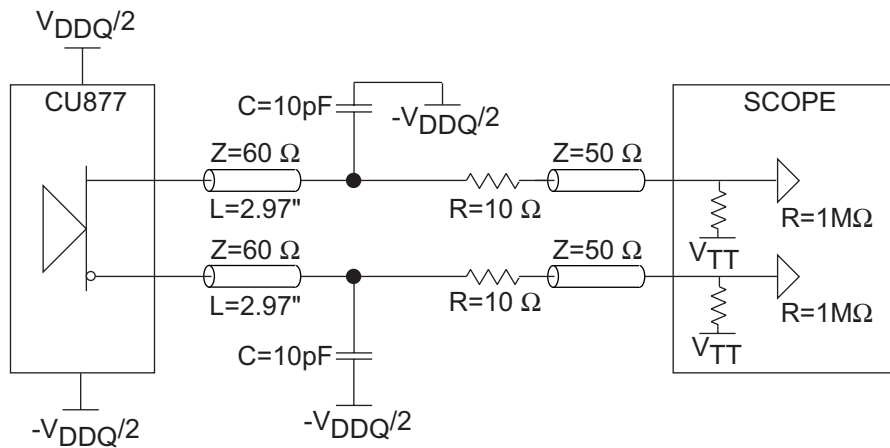
Figure 3. Output Load Test Circuit 1
