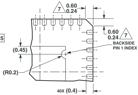
DETAIL M PREFERRED BACKSIDE PIN 1 INDEX
