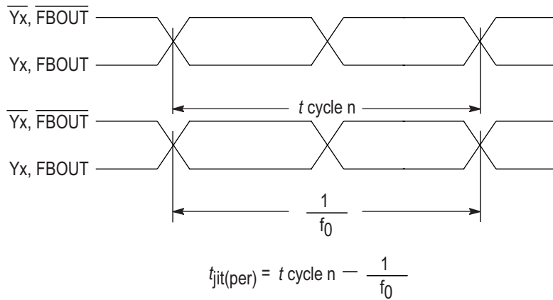
Figure 8. Period Jitter
