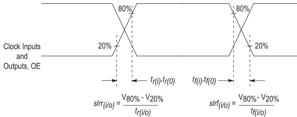
Figure 10. Input and Output Slew Rates
