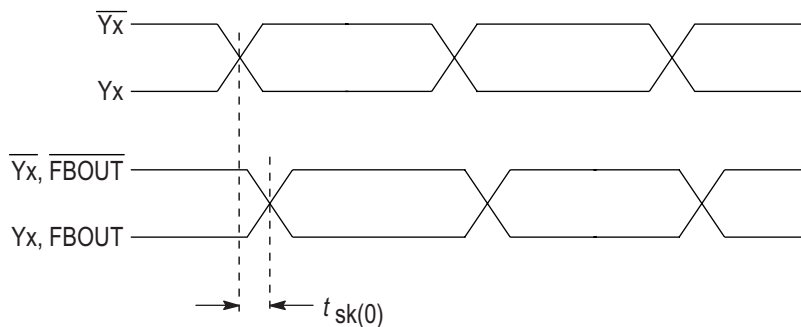
Figure 7. Output Skew
