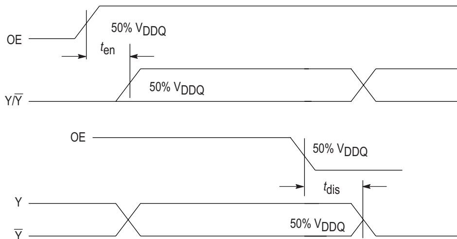
Figure 12. Time Delay between OE and Clock Output
