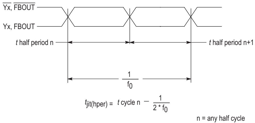
Figure 9. Half-Period Jitter
