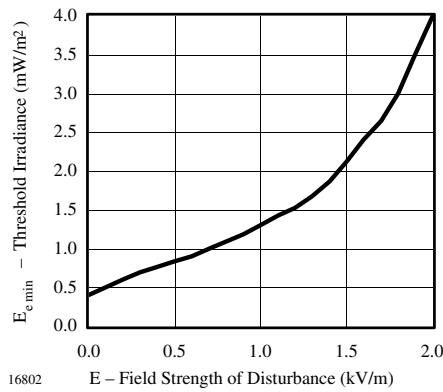
Figure 4. Threshold Irradiance vs. Field Strength of Disturbance
