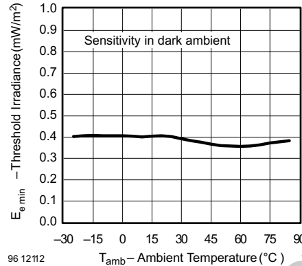
Figure 6. Sensitivity vs. Ambient Temperature
