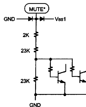
(6) MUTE equivalent circuit
