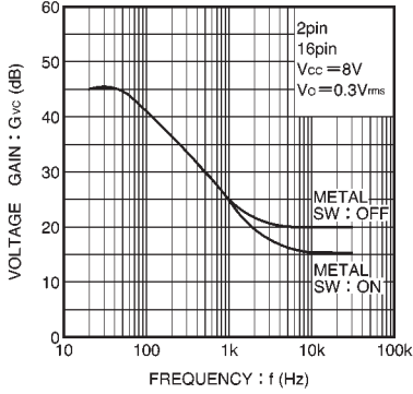
Fig. 8 Metal tape equalizer characteristics
