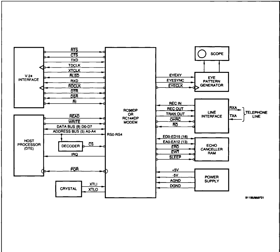
Figure 1. Modem Functional Interconnect Diagram
