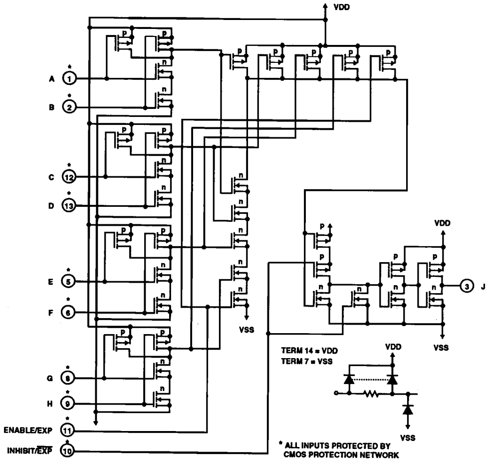
FIGURE 1. SCHEMATIC DIAGRAM
