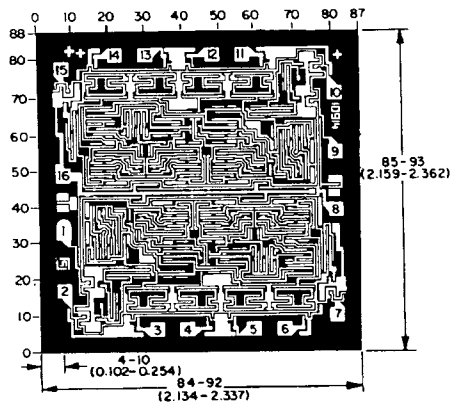
CD4518BMS
