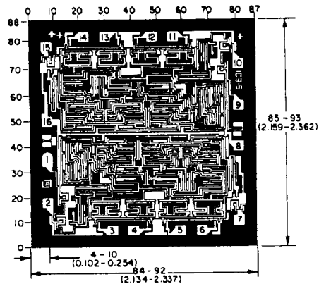
CD4520BMS
