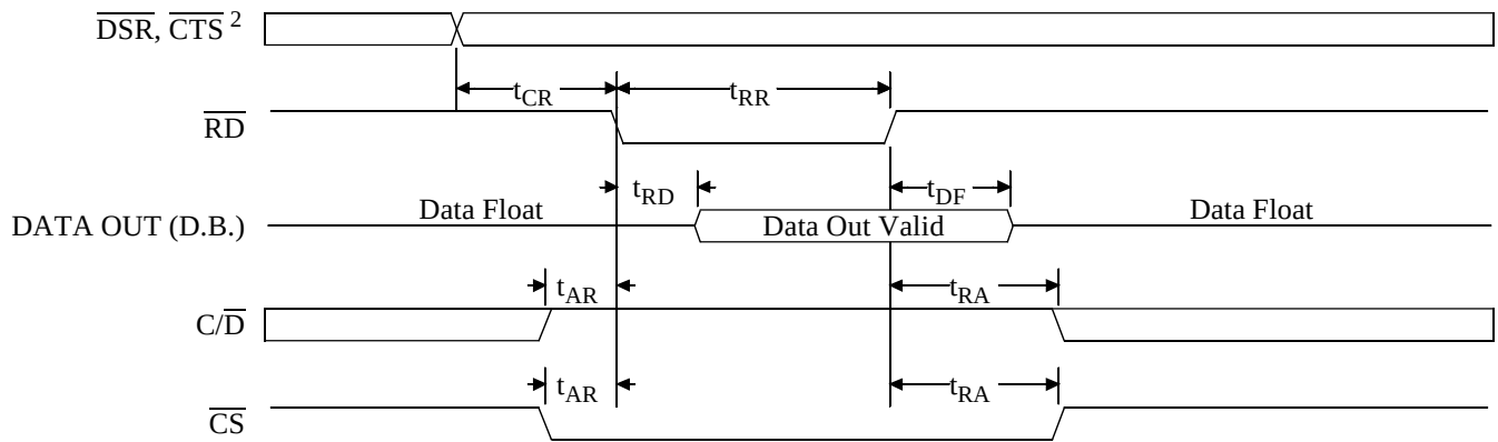
Figure 26. \overline{RD} CONTROL
