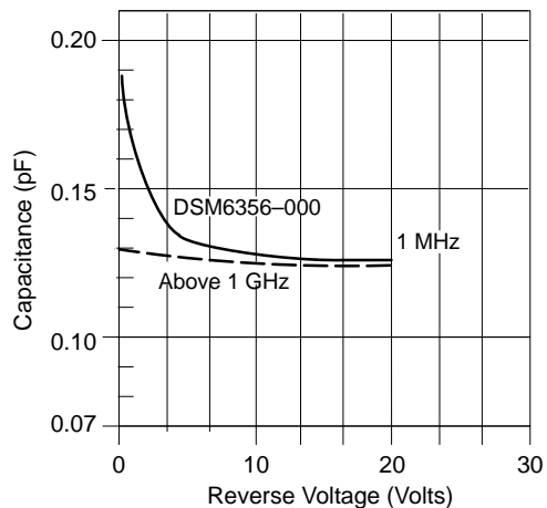
Figure 22. Typical Capacitance vs. Reverse Voltage
