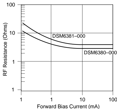
Figure 16. Typical RF Resistance vs. Forward Bias Current for DSM6380-000 and DSM6381-000
