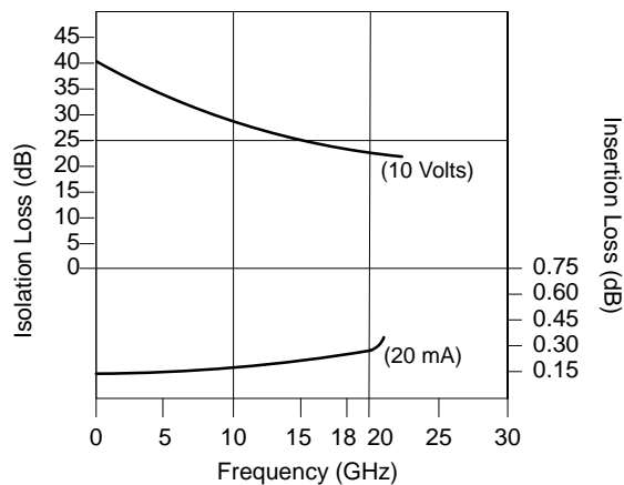
Figure 4. Typical Insertion Loss and Isolation Characteristics
