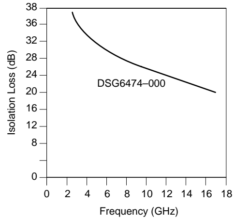
Figure 7. Isolation vs. Frequency, SPDT DSG6474-000
