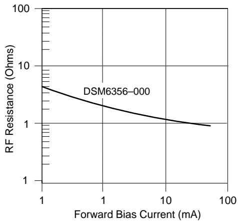
Figure 21. Typical RF Resistance vs. Forward Bias Current
