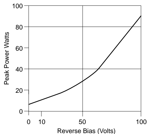
Figure 11. Peak Power Handling, SPST, 1 GHz DSG6474-000
