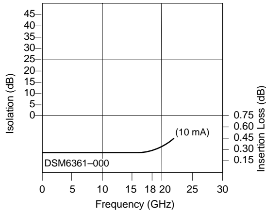
Figure 17. Typical Isolation and Insertion Loss Characteristics of the DSM6361-000
