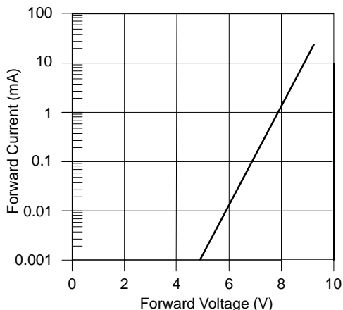
Figure 13. Typical Forward Characteristics of the DSM6380-000
