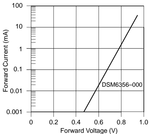
Figure 20. Typical Forward Characteristics
