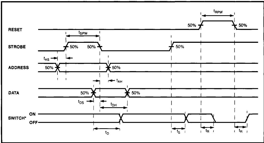
Figure 3 - Control Memory Timing Diagram
