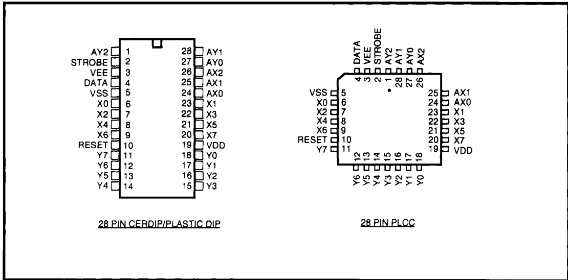
Figure 2 - Pin Connections
