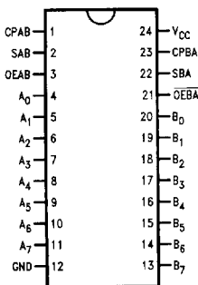
Pin Assignment DIP, SOIC and Flatpak
