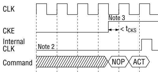
2) Power Down (= Precharge Power Down) Exit
