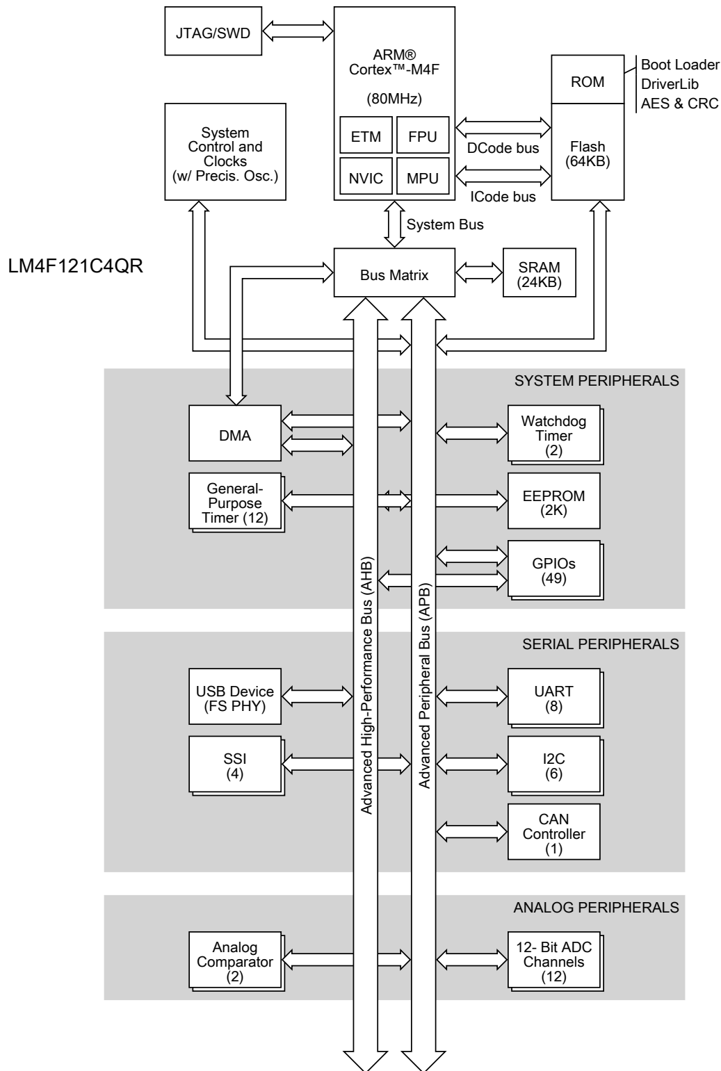
Figure 1-2. Stellaris LM4F121C4QR Microcontroller High-Level Block Diagram
