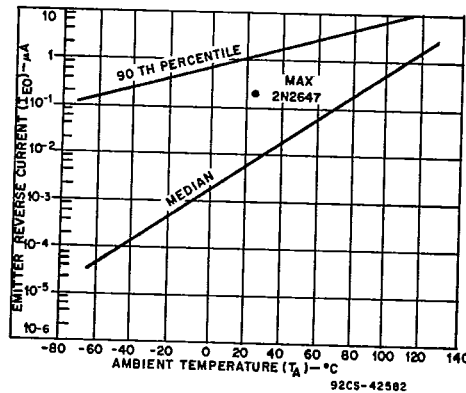
Fig. 7—Typical emitter reverse current characteristics.
