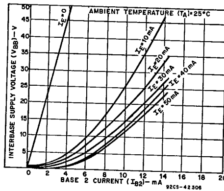
Fig. 5—Typical static interbase characteristics
