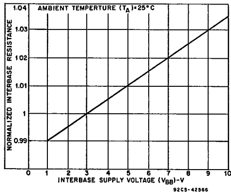
Fig. 13 - Normalized interbase resistance characteristic.
