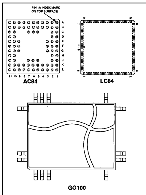
Fig.1 Pin connections - bottom view
