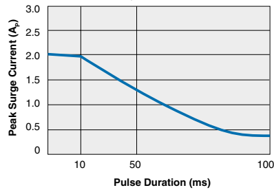
CPC1962G Maximum Surge Current (non-repetitive) ( T_J = 50^\circ\text{C} max)
