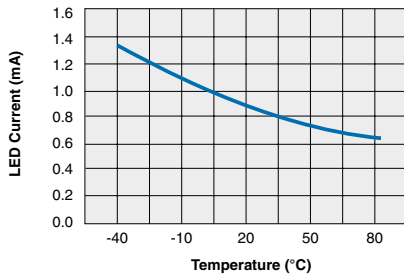
CPC1962G Typical I_F for Switch Operation vs. Temperature
