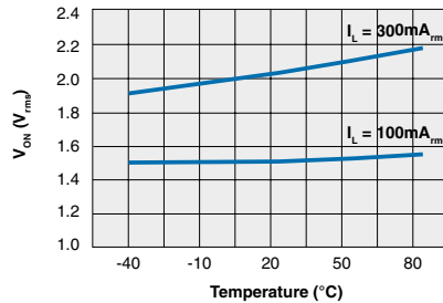
CPC1962G Typical Output Voltage Drop vs. Temperature
