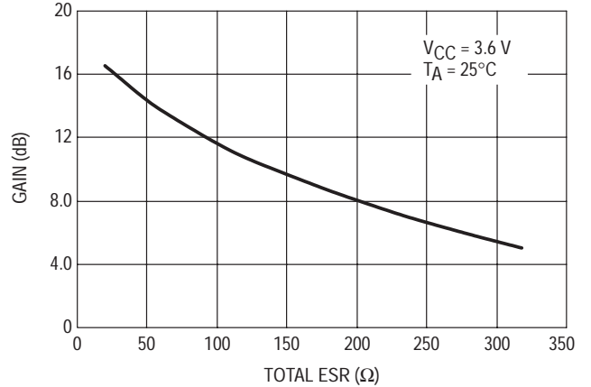
Figure 40. Reference Oscillator Open Loop Gain versus ESR
