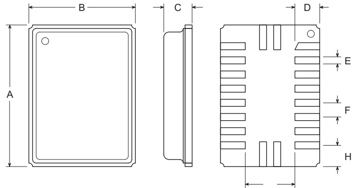
SM-20H Pac age Drawing
