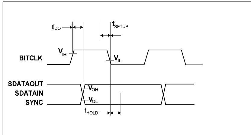
Figure 8 Data Setup and Hold (50pF External Load)
