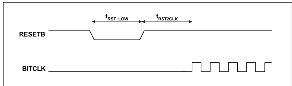
Figure 5 Cold Reset Timing
