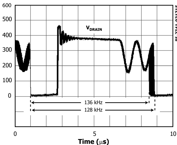
Figure 4. Frequency Jitter.
