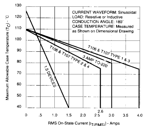
Figure 1B — Maximum Allowable Case Temperature vs RMS On-State Current
