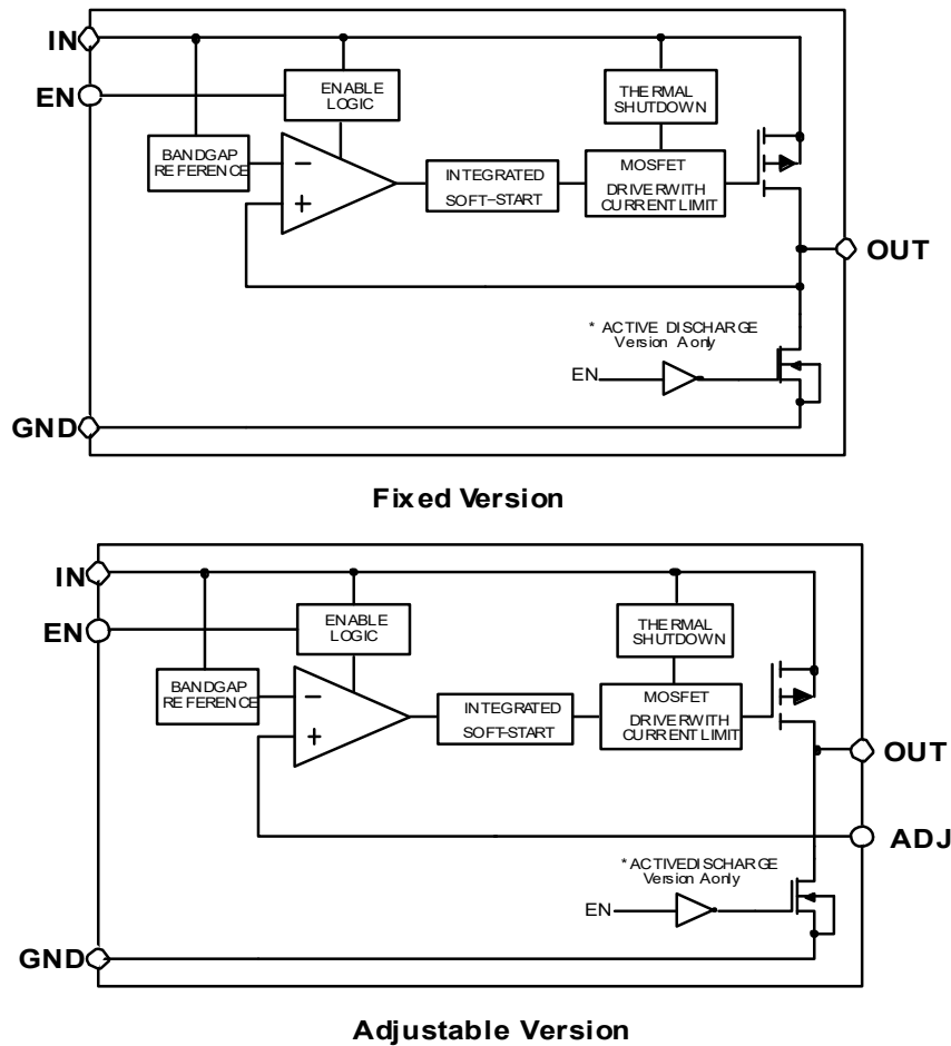
Figure 13. Functional Block Diagram
