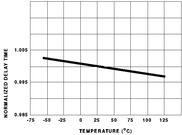
FIGURE 14. DELAY TIME vs TEMPERATURE
