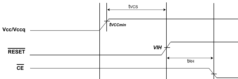
Figure 3: Vcc Power-up Diagram
