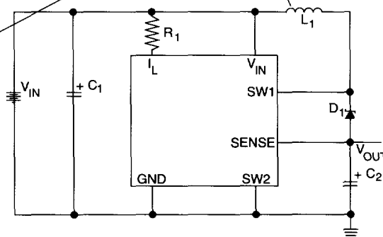
Boost converter
