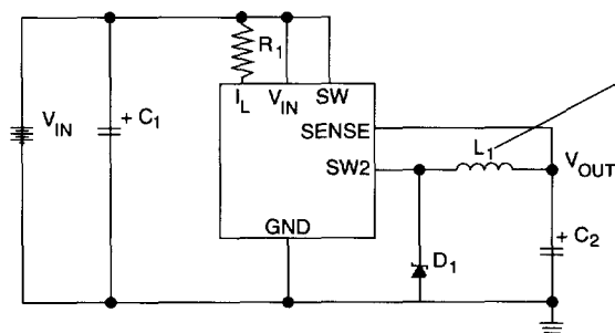
Buck converter
