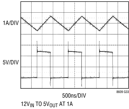
Switching Waveforms
