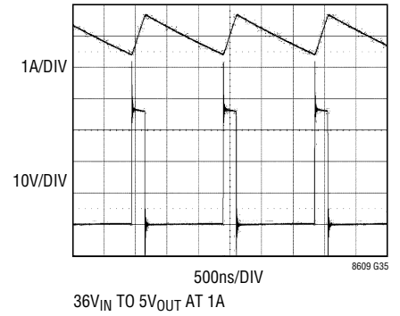
Switching Waveforms
