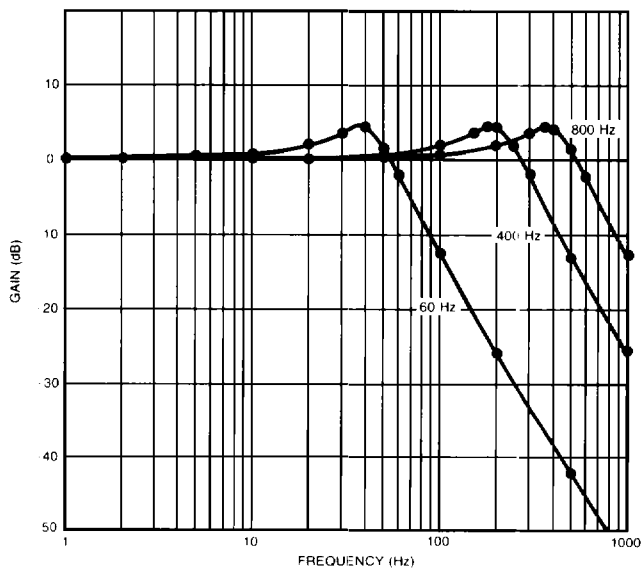
FIGURE 22 Gain Plot (1044)
