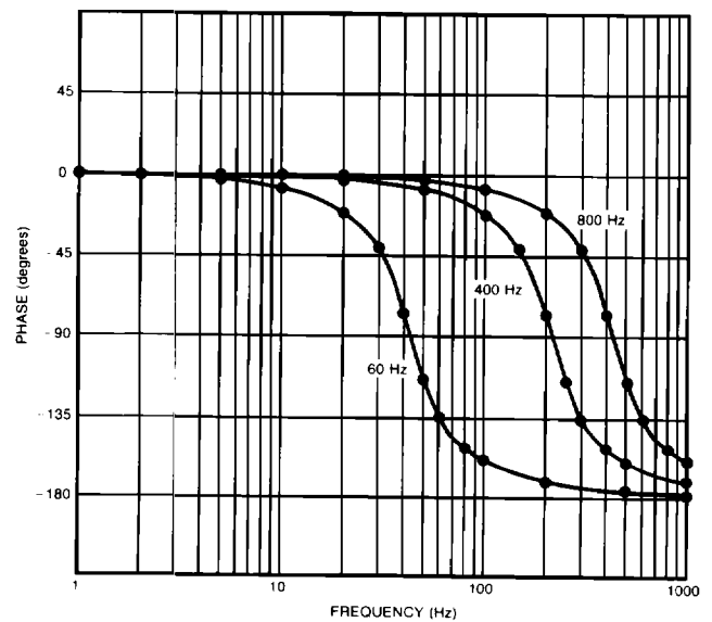
FIGURE 23 Phase Plot (1044)
