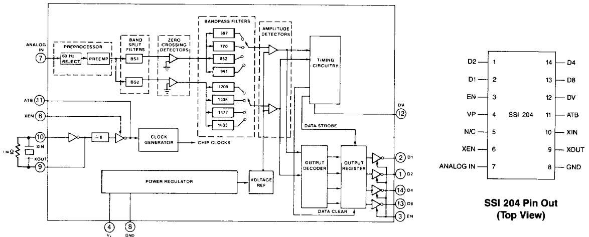
Block Diagram
