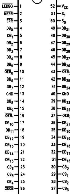
Pin Assignment for Side Brazed DIP
