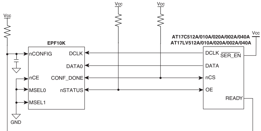
Figure 1. Configuration with a Single AT17A Series Configurator
