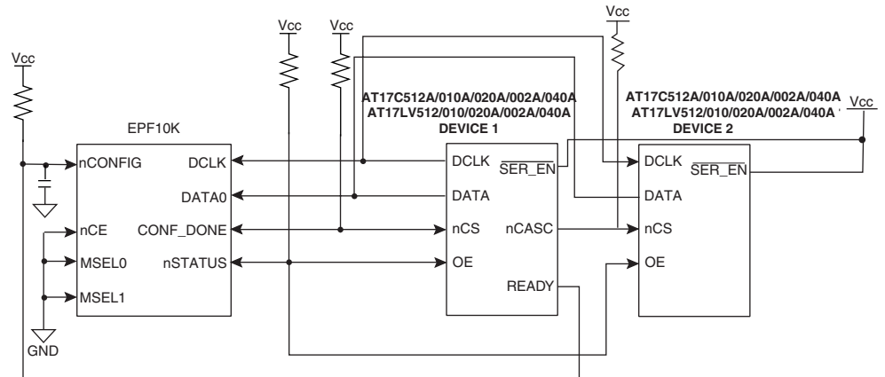
Figure 2. Configuration with Multiple AT17A Series Configurators
