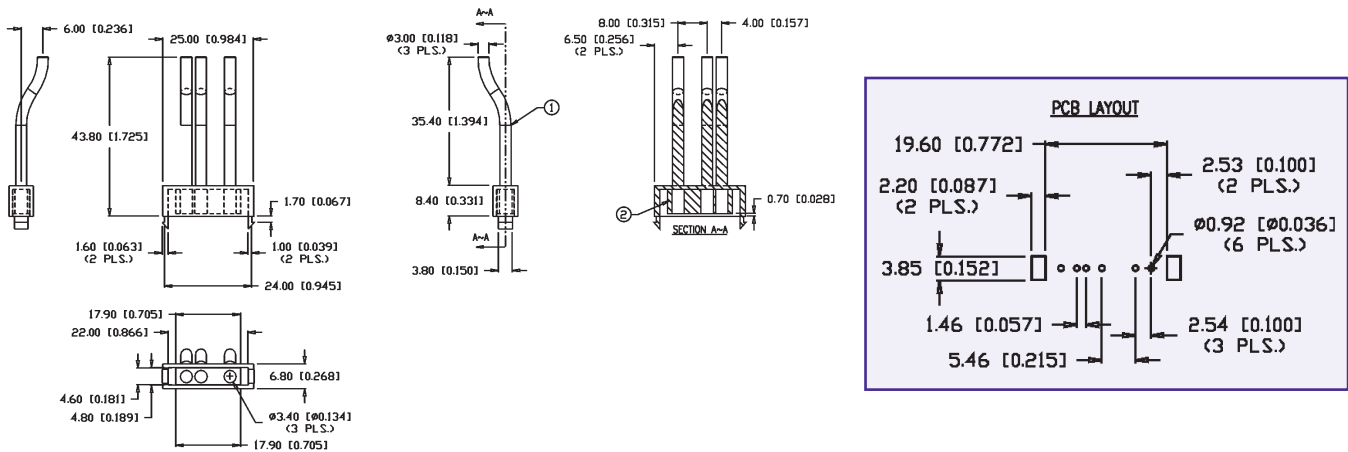
Figure 42 Part # LPA-C051301S-6
