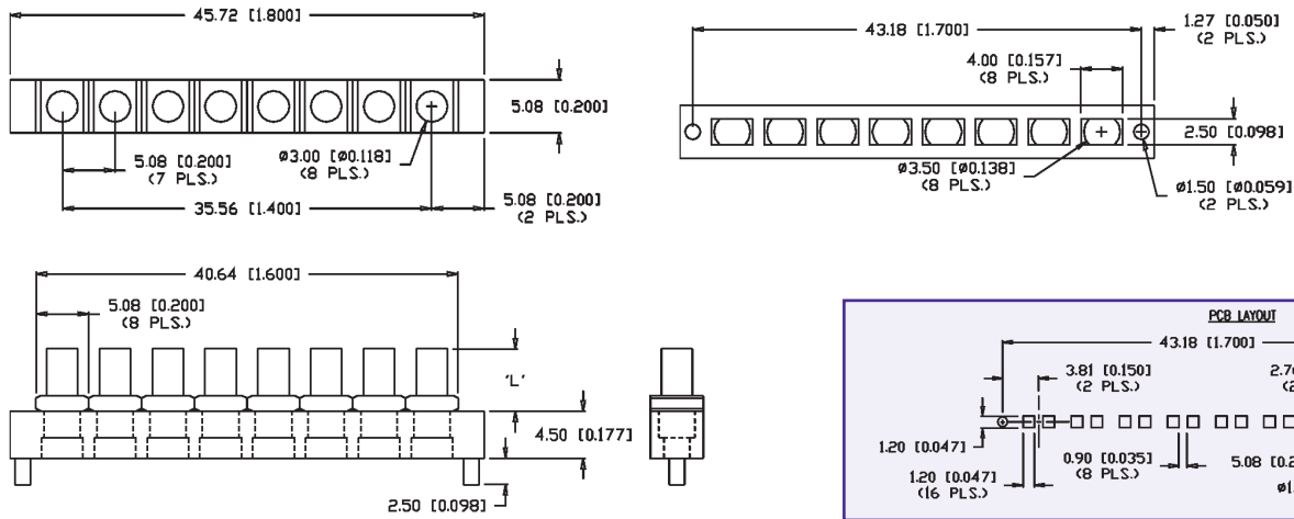
Figure 41 Part # LPA-C031301D-35
