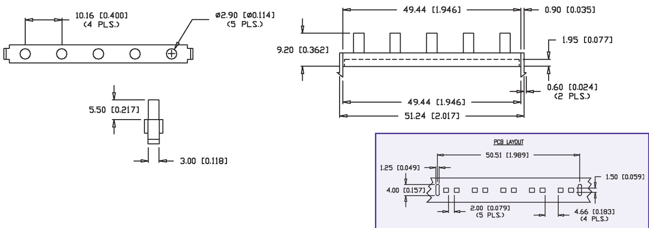
Figure 42 Part # LPA-C051301S-6
