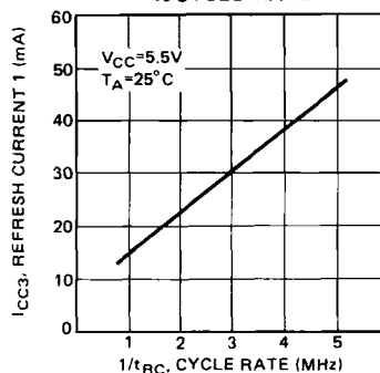
Fig. 10 – REFRESH CURRENT 1 vs CYCLE RATE
