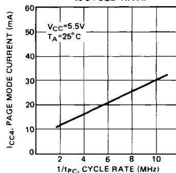
Fig. 12 – PAGE MODE CURRENT vs CYCLE RATE
