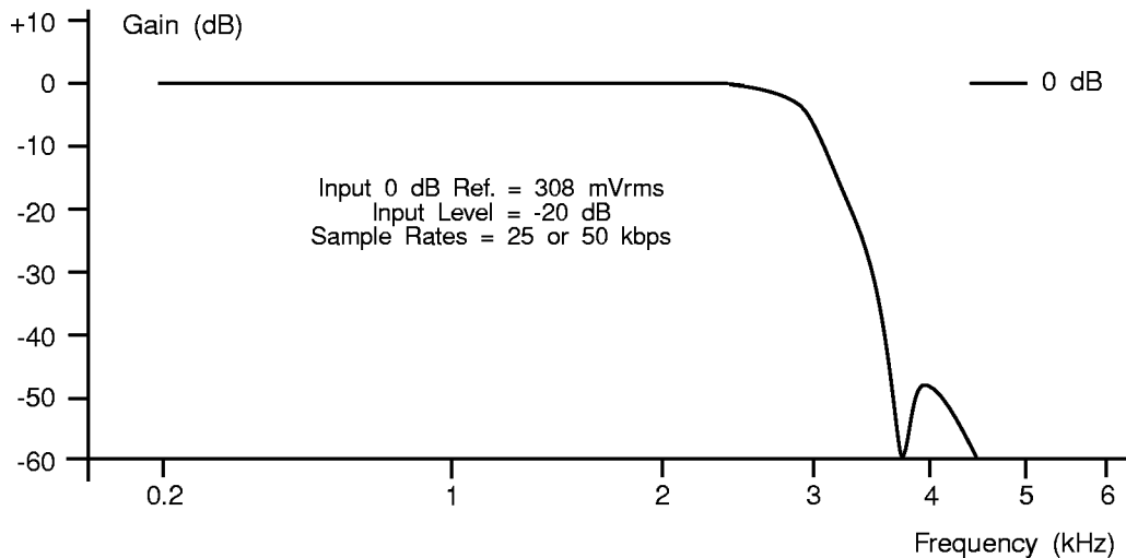
Figure 8: Typical Overall (Encoder + Decoder) Frequency Response
