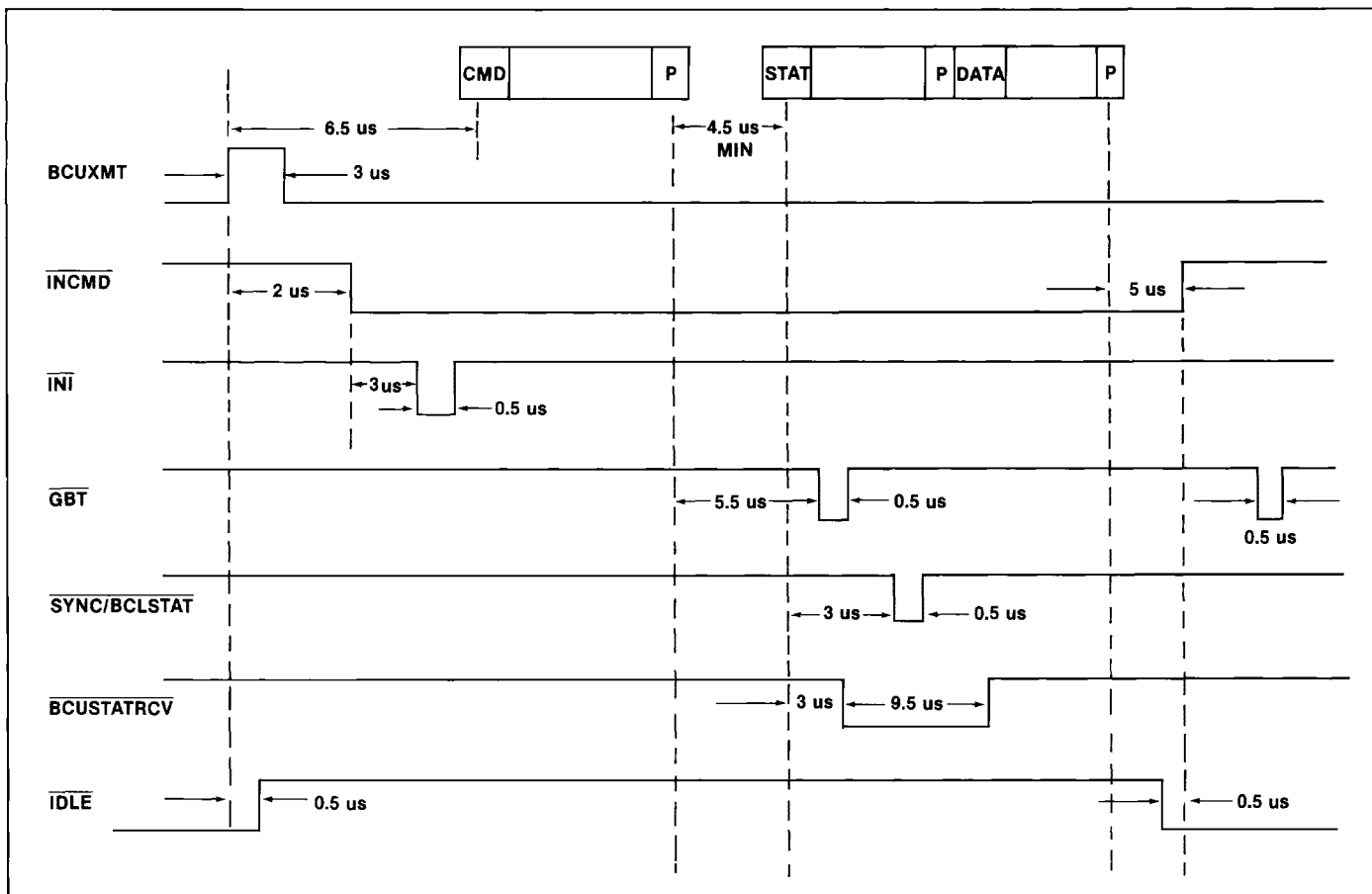
Figure 4d: Transmit Command-Bus Controller Mode
