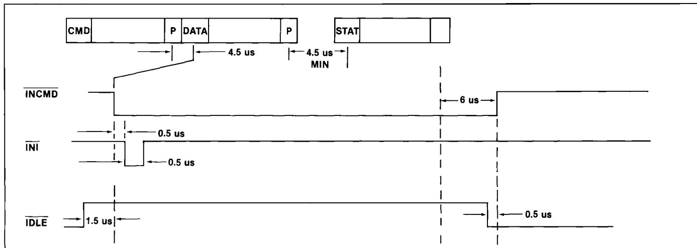
Figure 4e: Bus Monitor-Receive Message
