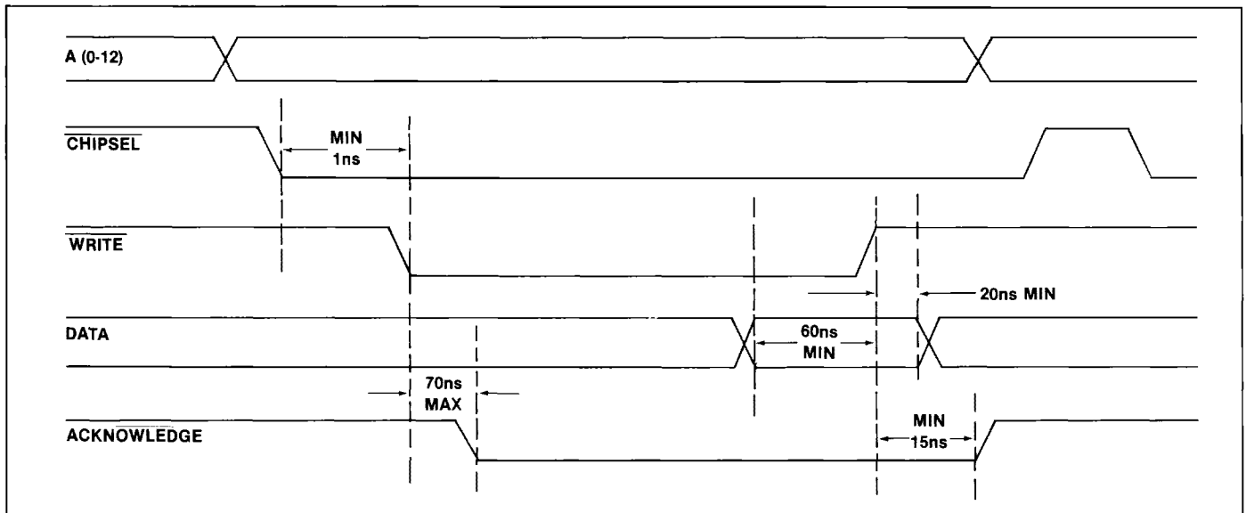
Figure 4g: Write Memory
