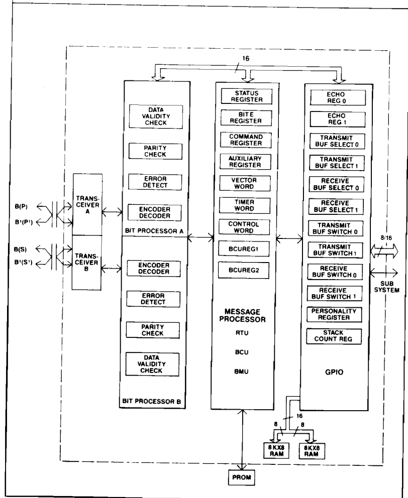
Figure 1: Universal Bus Interface Unit - Block Diagram
