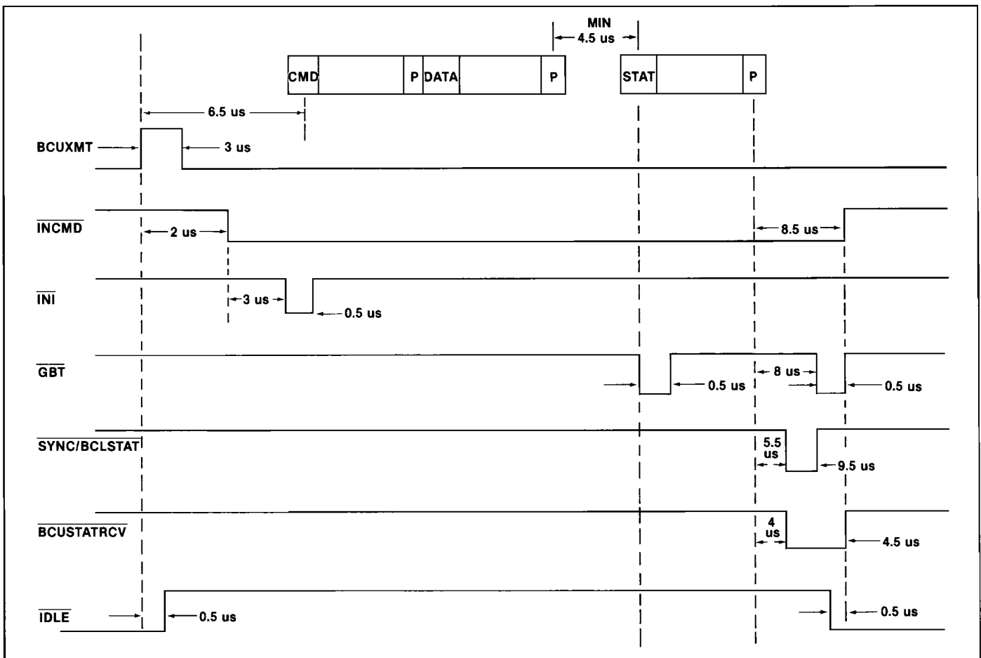
8 Figure 4c: Receive Command - Bus Controller Mode
