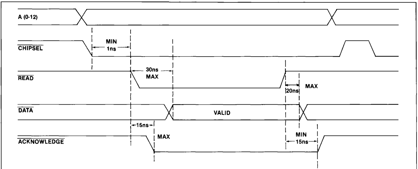
Figure 4f: Read Memory
