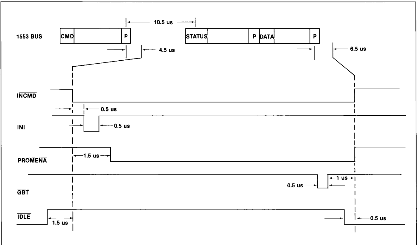
Figure 4b: Transmit Timing Diagram - Remote Terminal Mode
