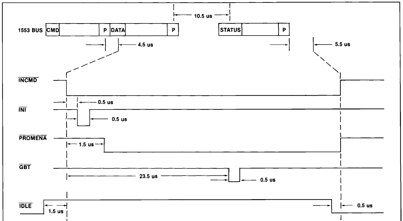
Figure 4a: Receive Timing Diagram—Remote Terminal Mode
