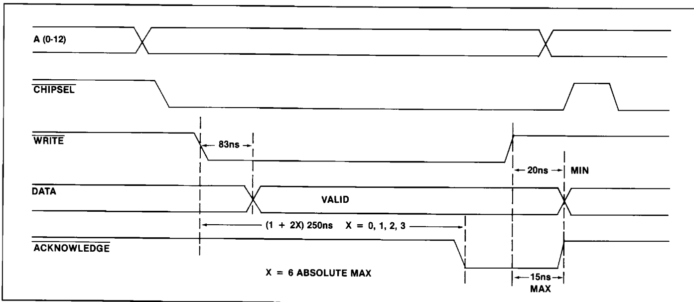
Figure 4i: MP Register Write
