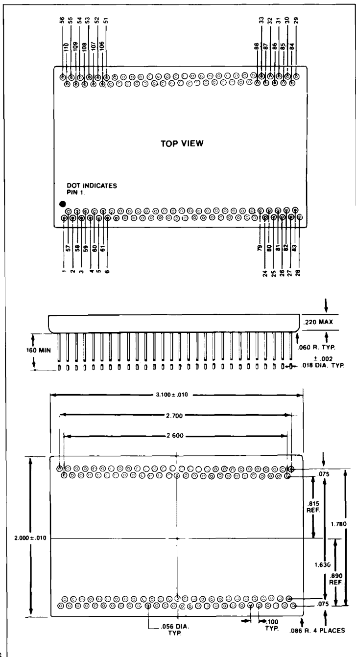
Figure 2: Mechanical Outline 110 Pins
