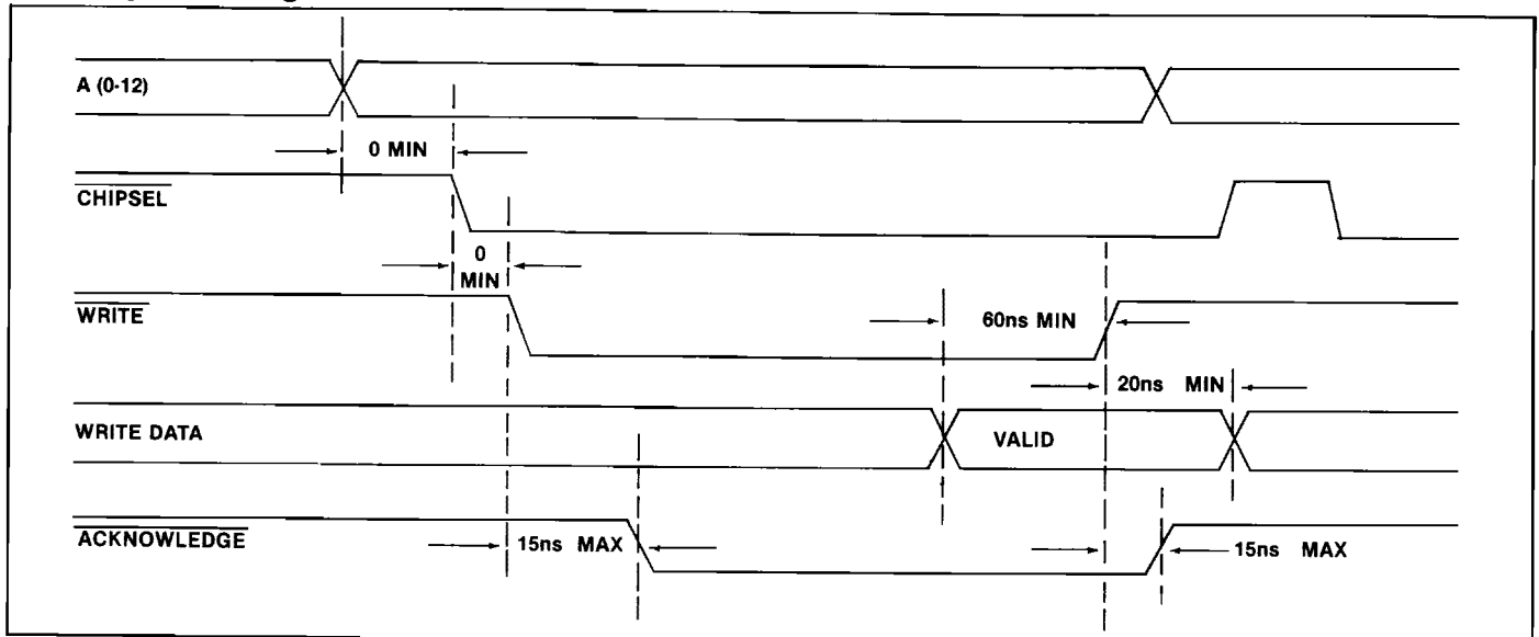
Figure 4k: GPIO Register Write
