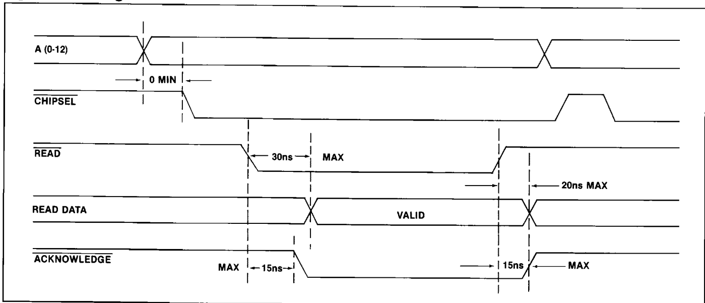
Figure 4j: GPIO Register Read
