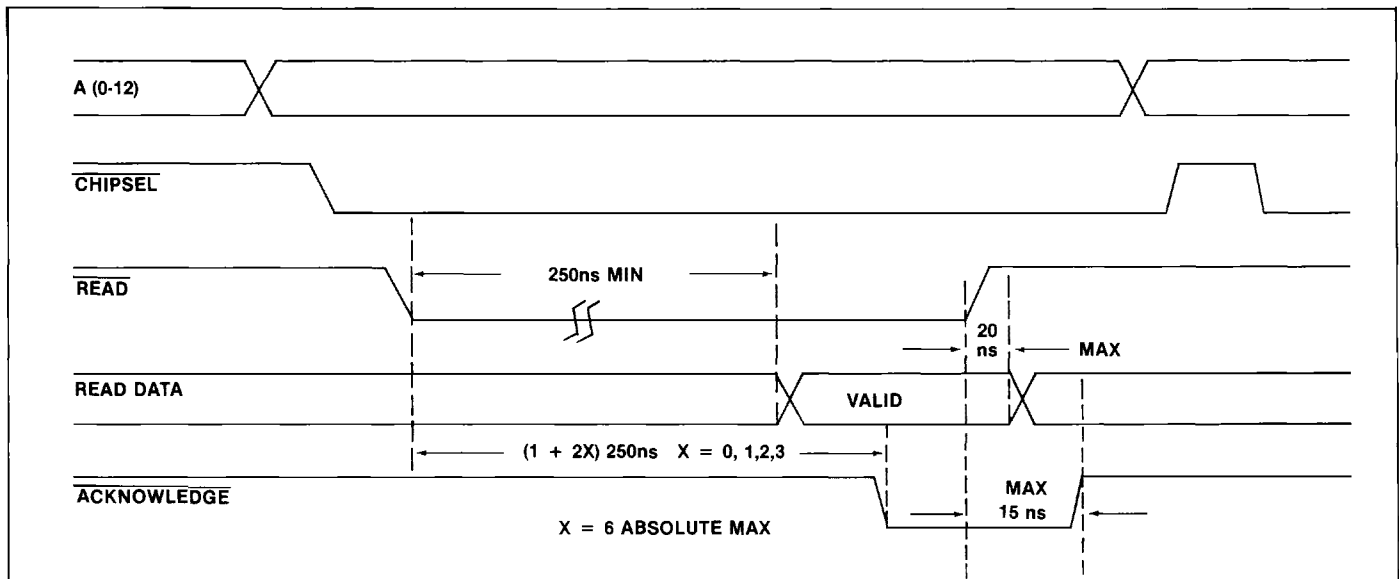
10 Figure 4h: MP Register Read
